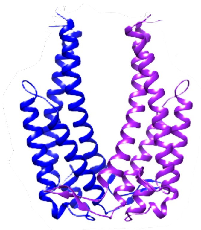
Figure 6: 3D- Model of OspC from B. afzelii
