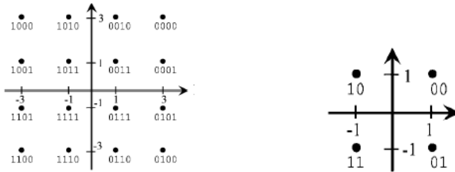
Figure.2-9 : Mapping cells into constellation diagrams: (a) 16QAM, (b) QPSK [2]
