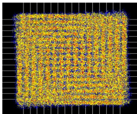
(b)MER=22.4 dB
