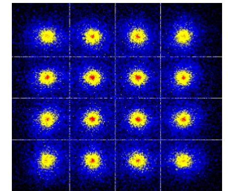
(f)MER=13.5dB
