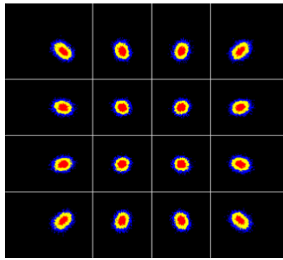
(a)MER=29.3dB
