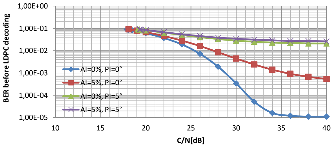
Figure.1: BER before LDPC decoding vs. C/N in AWGN channel(scenario1)
