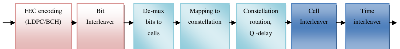
Figure.2-5:Bit Interleaved Coding and Modulation (BICM) ( based on [2])
