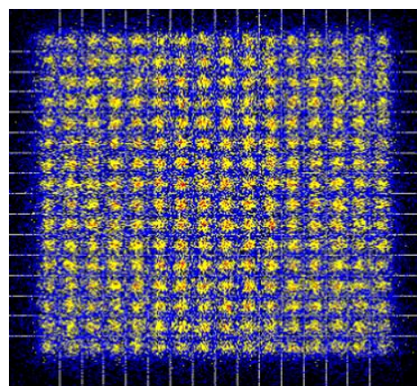
(f)MER=16.2 dB
