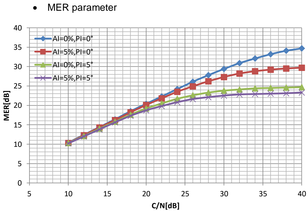
Figure.10: MER vs C/N in the AWGN channel (scenario2)
