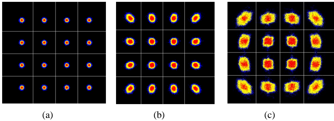
Figure.3. 3: 16-QAM constellation diagrams : (a) AI=0%,PI=0° (b) AI=10%,PI=0°(c) AI=0%,PI=10°
