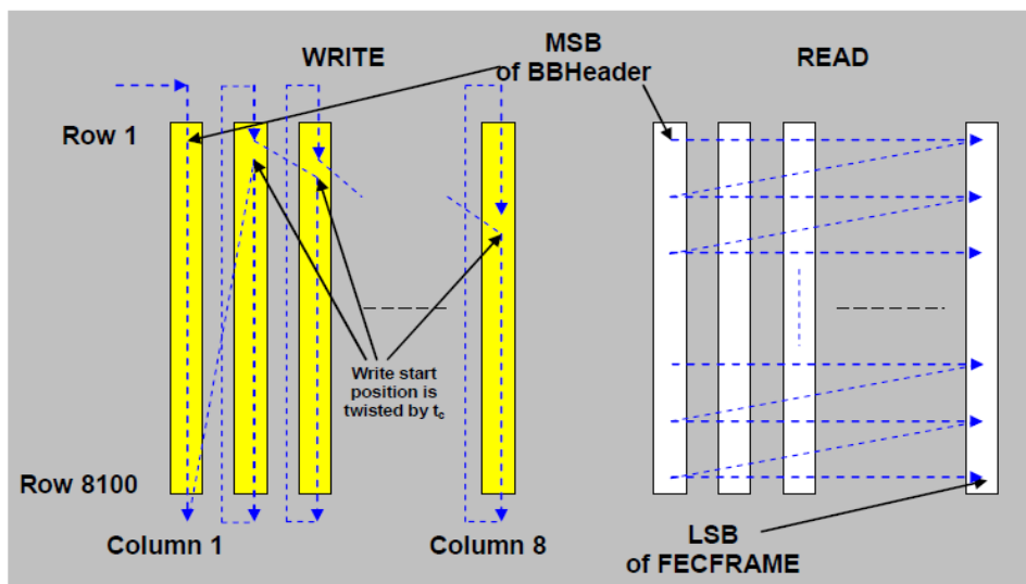
Figure.2-7: Bit Interleaving [2]
