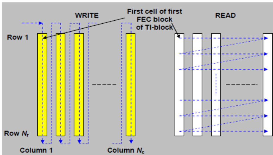
Figure.2-15 :Time interleaving[2]
