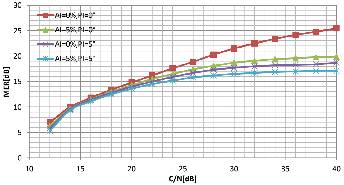
Figure.11: MER vs C/N in the RL20 channel (scenario2)
