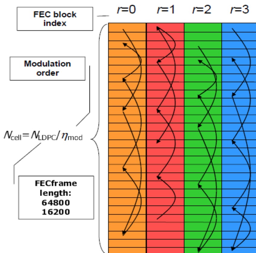
Figure. 2-11:Cell interleaving[3]
