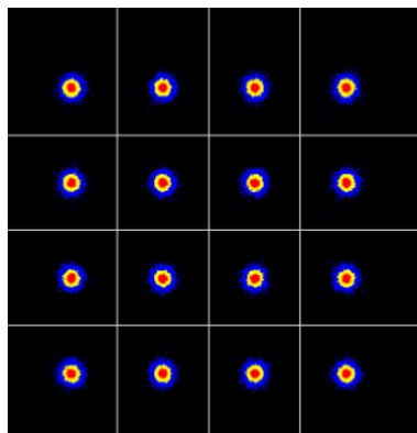
(c)MER=28.5 dB
