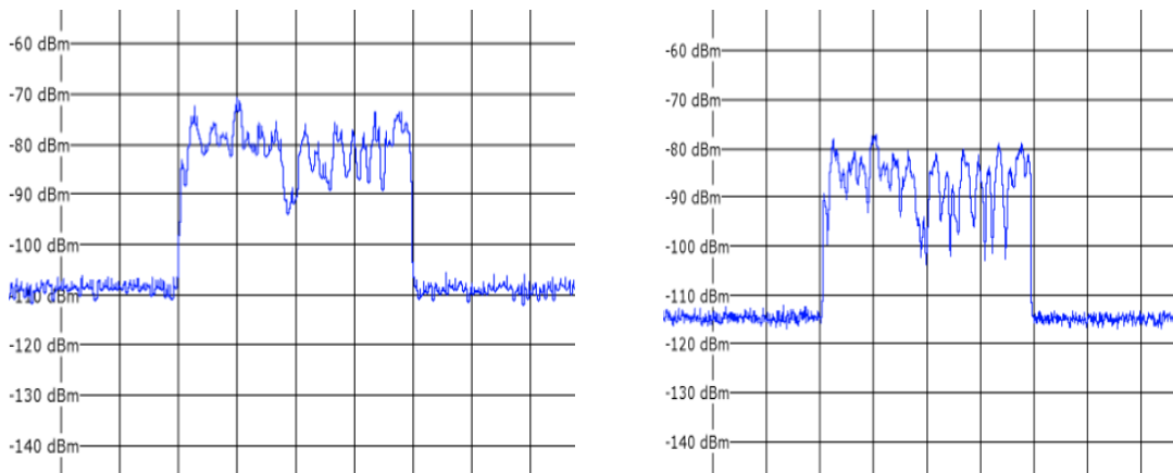
Figure.7: Snapshots of the 256-QAM spectrum diagrams in RL20 channel (a) AI=0%andPI=0° (b) AI=5%andPI=5°, All spectrum diagrams were captured at C/N=30 dB, Frequency =689 MHz, Span=20.0 Mhz, RBW= 100 KHz,VBW= 1MHZ
