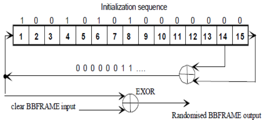
Figure.2-4:PRBS generator [2]
