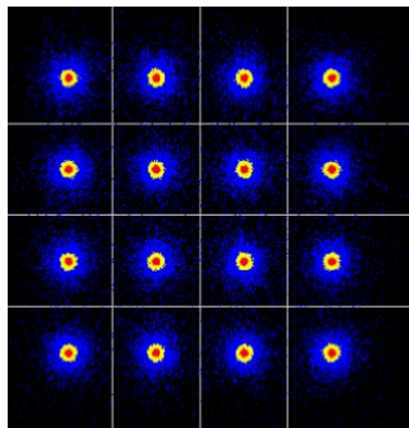
(e)MER=21.5 dB
