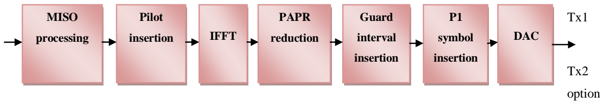
Figure.2-17:OFDM generation (based on[2])
