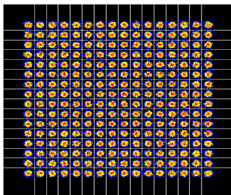
(a)MER=29.4 dB
