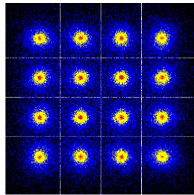
(f)MER=13.8 dB
