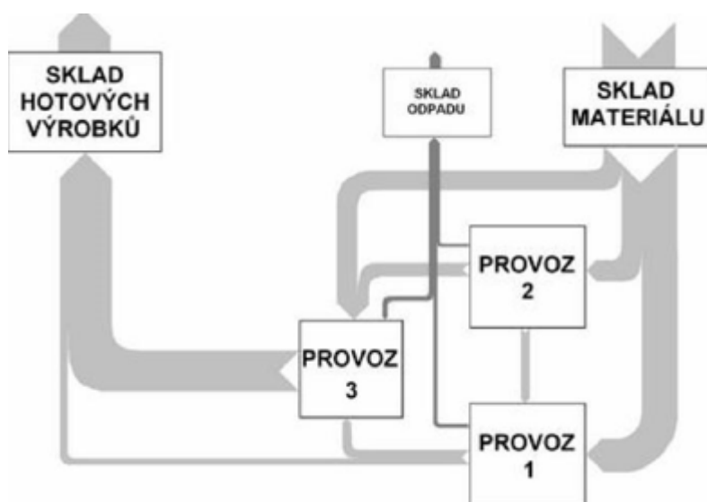
Obr. 1.4 Sankeyův diagram
