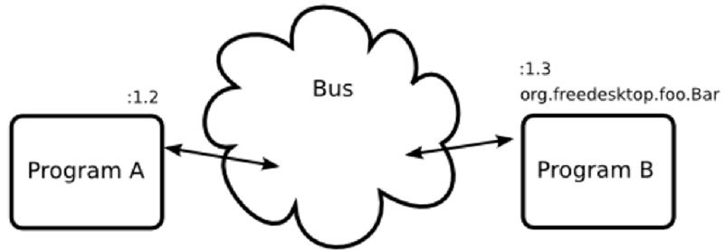
Figure 3.2: D-Bus id and well-known name example [7]
