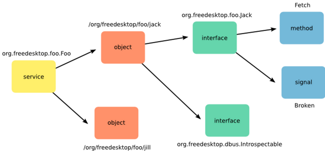
Figure 3.3: D-Bus architecture [7]
