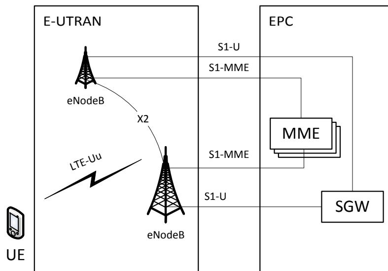
Figure 3.1 E-UTRA
