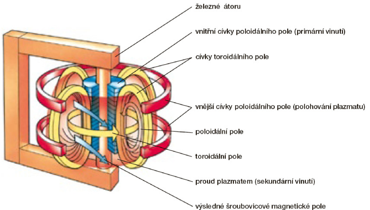
Obr. 1-1 schéma tokamaku [4]
