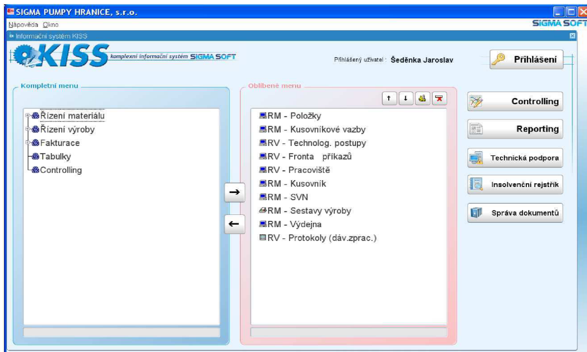
Obr. 2.22 Program Kiss.
