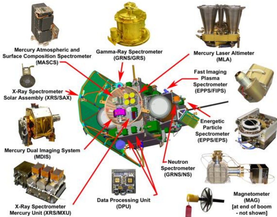
Figure 5: MESSENGER payload instruments and their location
