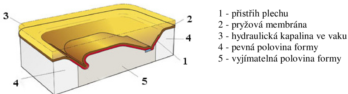
Obr. 10 Princip metody Flexform [2]
