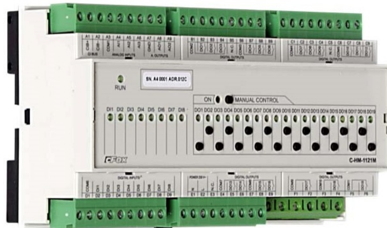
Obr. 4.3: Modul C-HM-1121M
