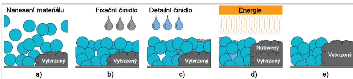
Obr. 2 Schéma principu technologie Multi jet fusion [21]
