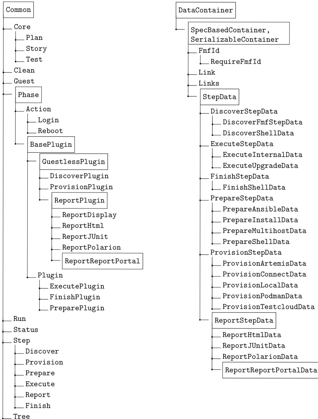
Figure 4.3: Inheritance of tmt method classes Figure 4.4: Inheritance of tmt data classes
