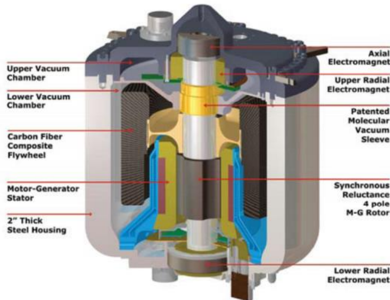
Figure 10 Cross section of flywheel [22]
