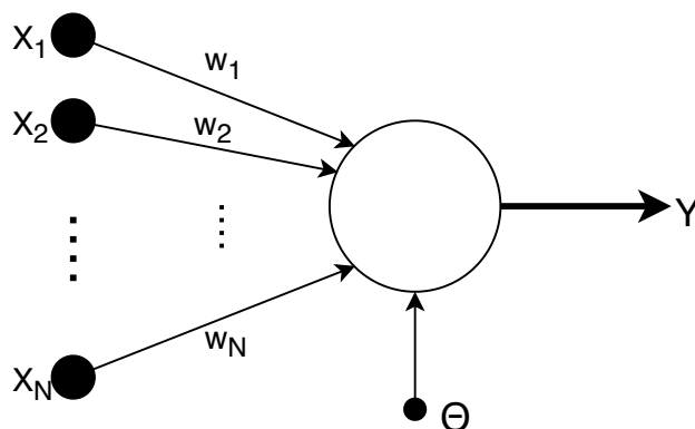
Obr. 1.1: Model neuronu
