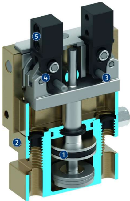
Obr. 81 Schunk GAP [22]
