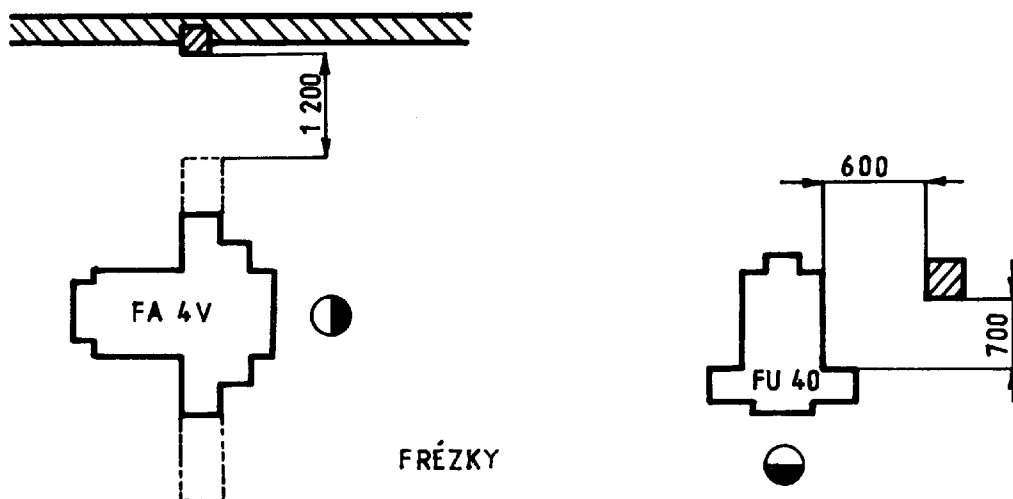
Obr. 1.11 Frézky. [10]
