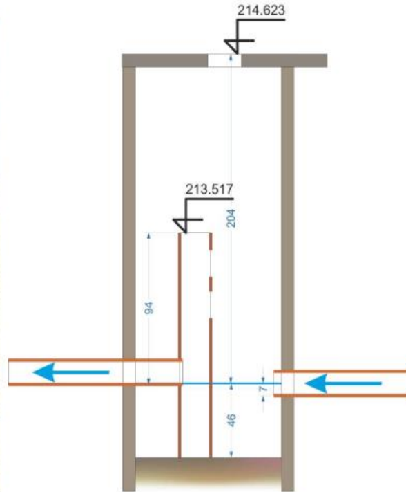
Figure 12: Reading the Exact localization of the control shaft by geodetical GPS. Source: Photo: K. Bářková; Scheme: V. David
