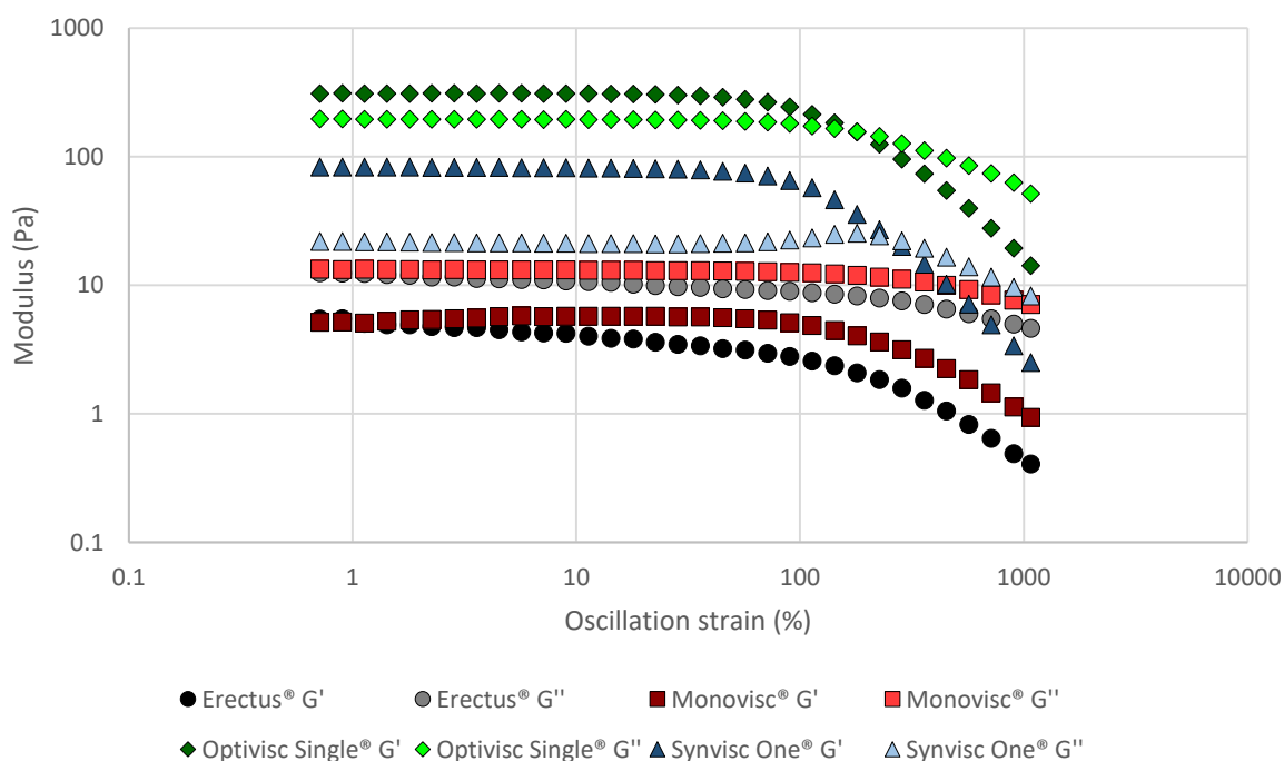
Figure 3 Dynamic modulus as a function of strain at \omega = 1 Hz
