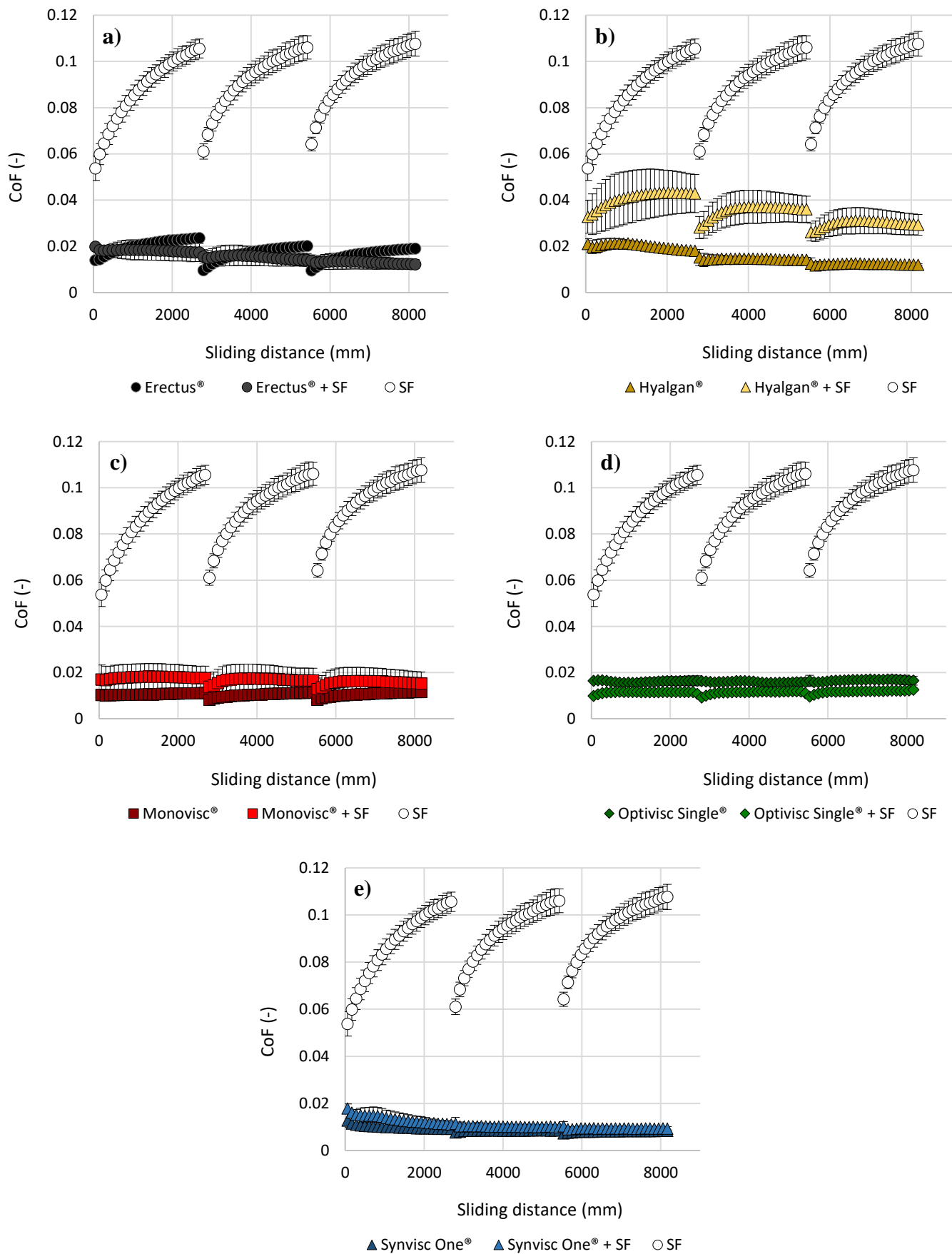
Figure 5 CoF as a function of the sliding distance for clear VSs and mixtures with model SF: a) Erectus®, b) Hyalgan®, c) Monovisc®, d) Optivisc Single®, e) Synvisc One®
