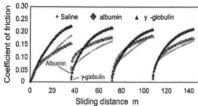
Figure 2-13 Influence of proteins on articular cartilage friction [22]
