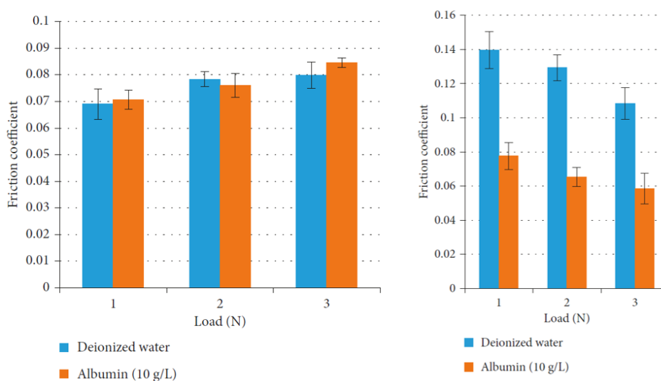
Figure 2-30 Effect of lubricant on CoF at a oscillating frequency of: a) 1 Hz, b) 2 Hz [41]
