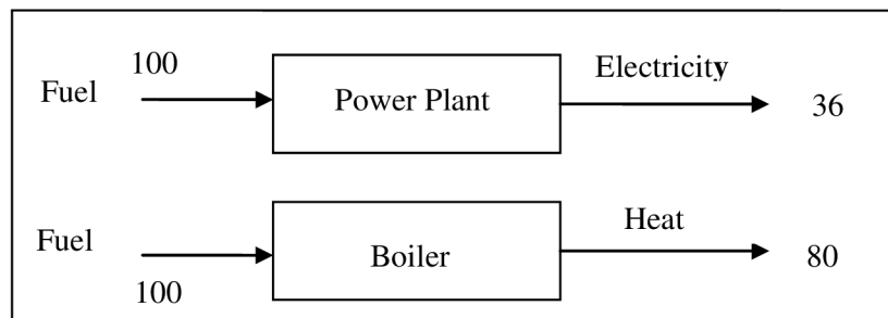
Fig. 8.3 Separate production of electricity and heat [23]
