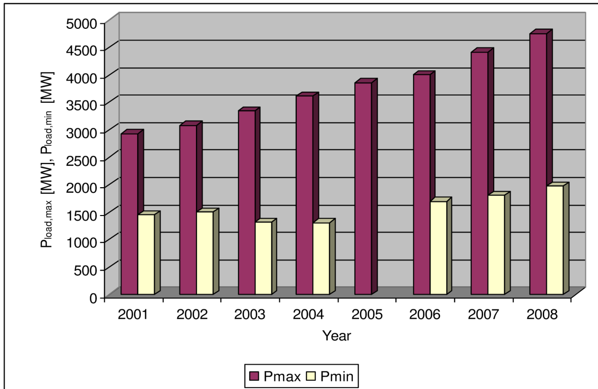
Fig. 4.11 Maximum and minimum load (2001-2008)
