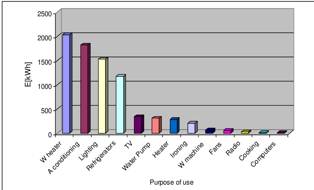
Fig. 11.1 Annually energy consumed depending on purpose of use of average consumer
