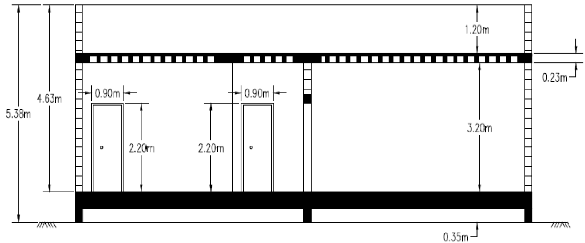
Fig. 11.14 Cross section A-A of building
