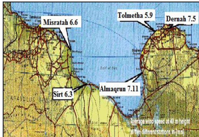
Fig. 4.6 Wind potential for Libyan coast area – average wind speed in m/s [11]
