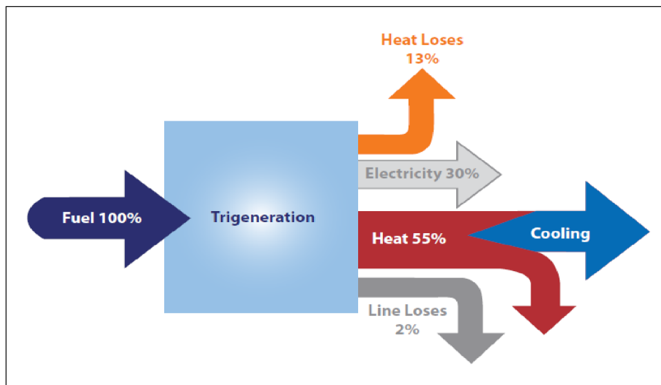
Fig. 9.1 Schematic diagram of Tri-generation process [24]
