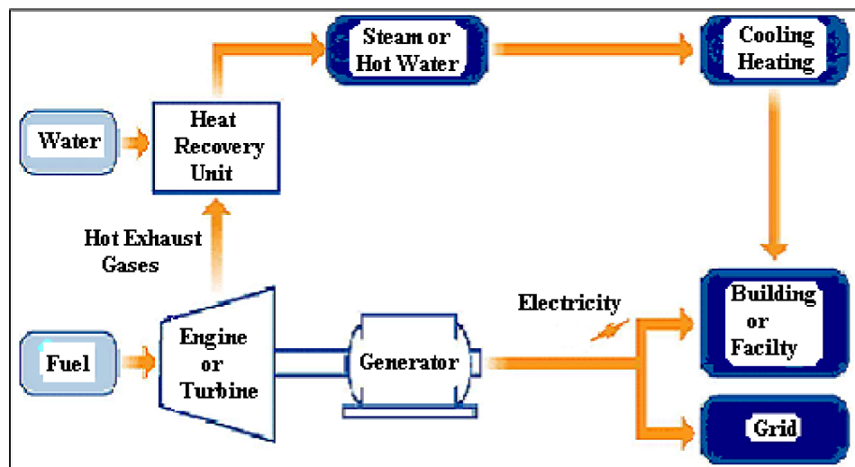
Fig. 8.2 Cogeneration with prime mover gas turbine or engine [21]
