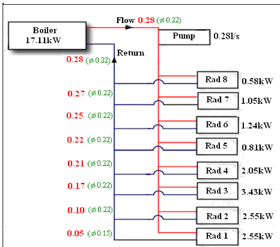
Fig. 11.17 Heating system of small house
