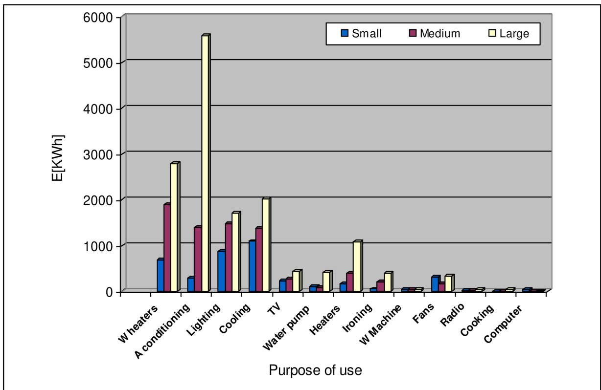
Fig. 11.4 Annual electrical energy consumption, depending of purpose of use, Sabha
