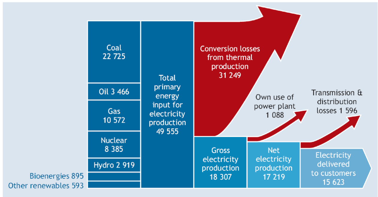
Fig. 2.2 Energy flows in the global electricity system [TWh][4]
