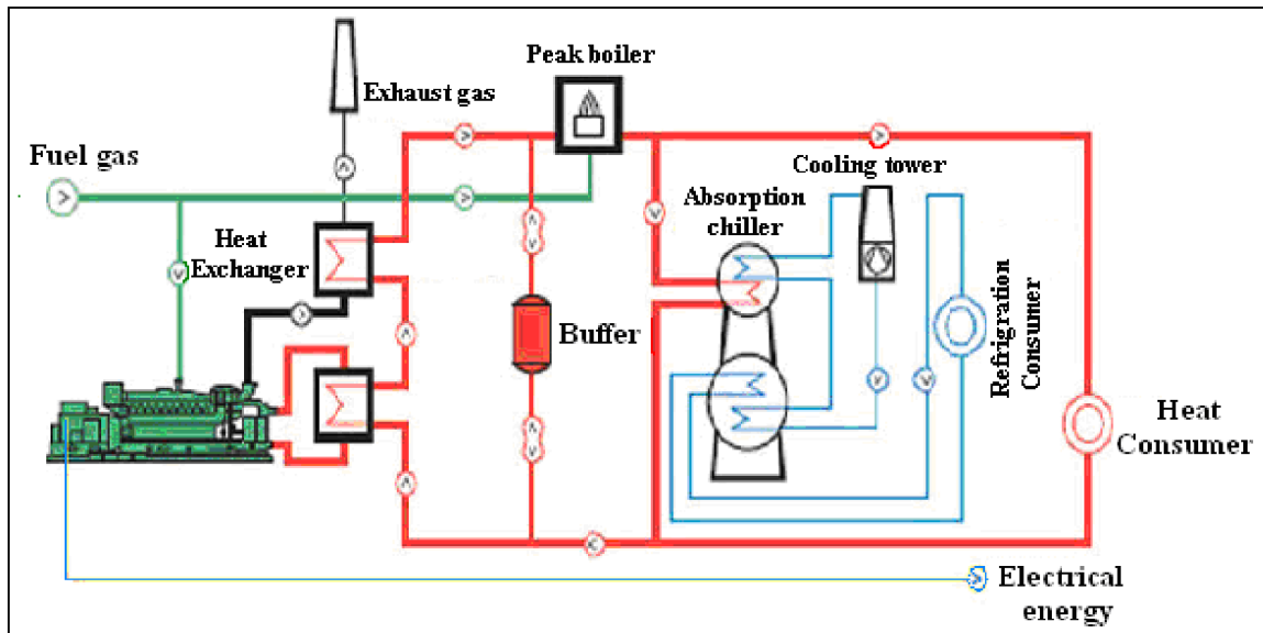
Fig. 9.2 Schematic showing overall tri-generation system configuration [24]
