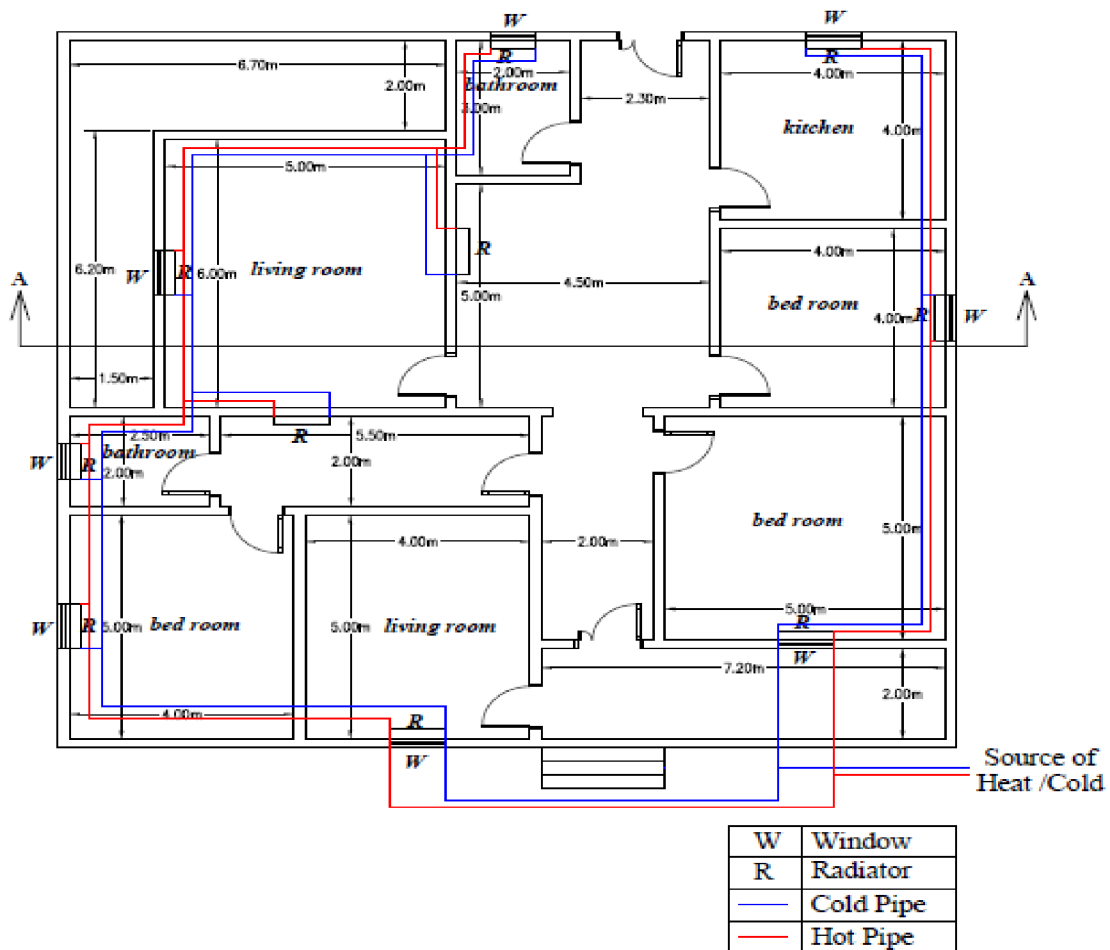
Fig. 11.18 Scheme for medium house
