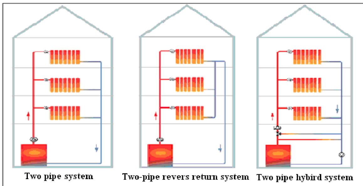
Fig. 11.9 Type of pipe distribution [43]
