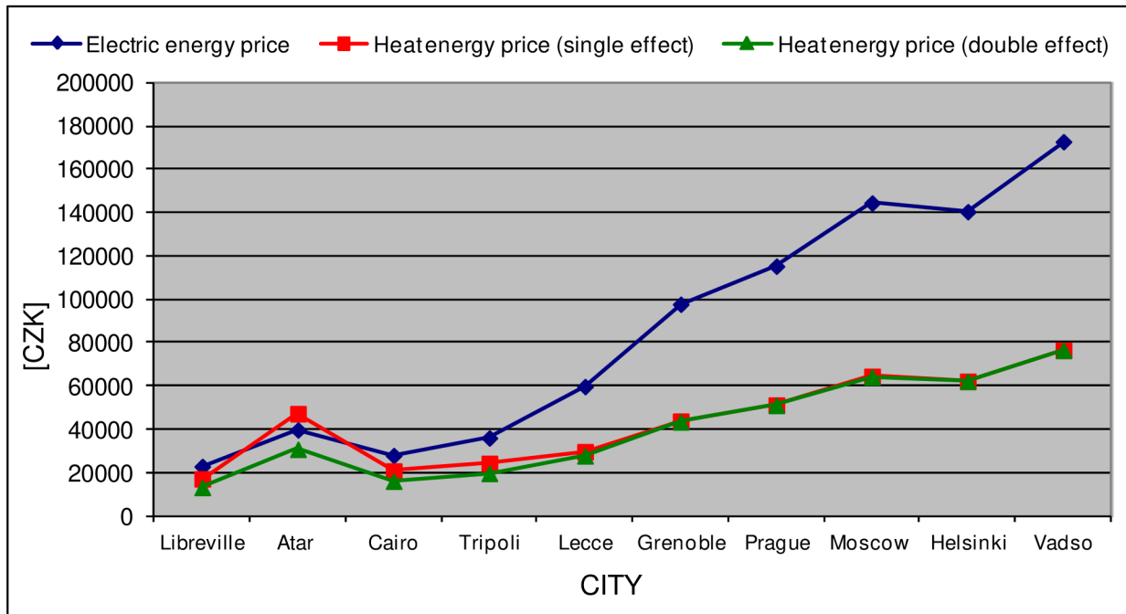
Fig. 12.4 Price in CZK of input energy (electrical & heat with single and double effect)
