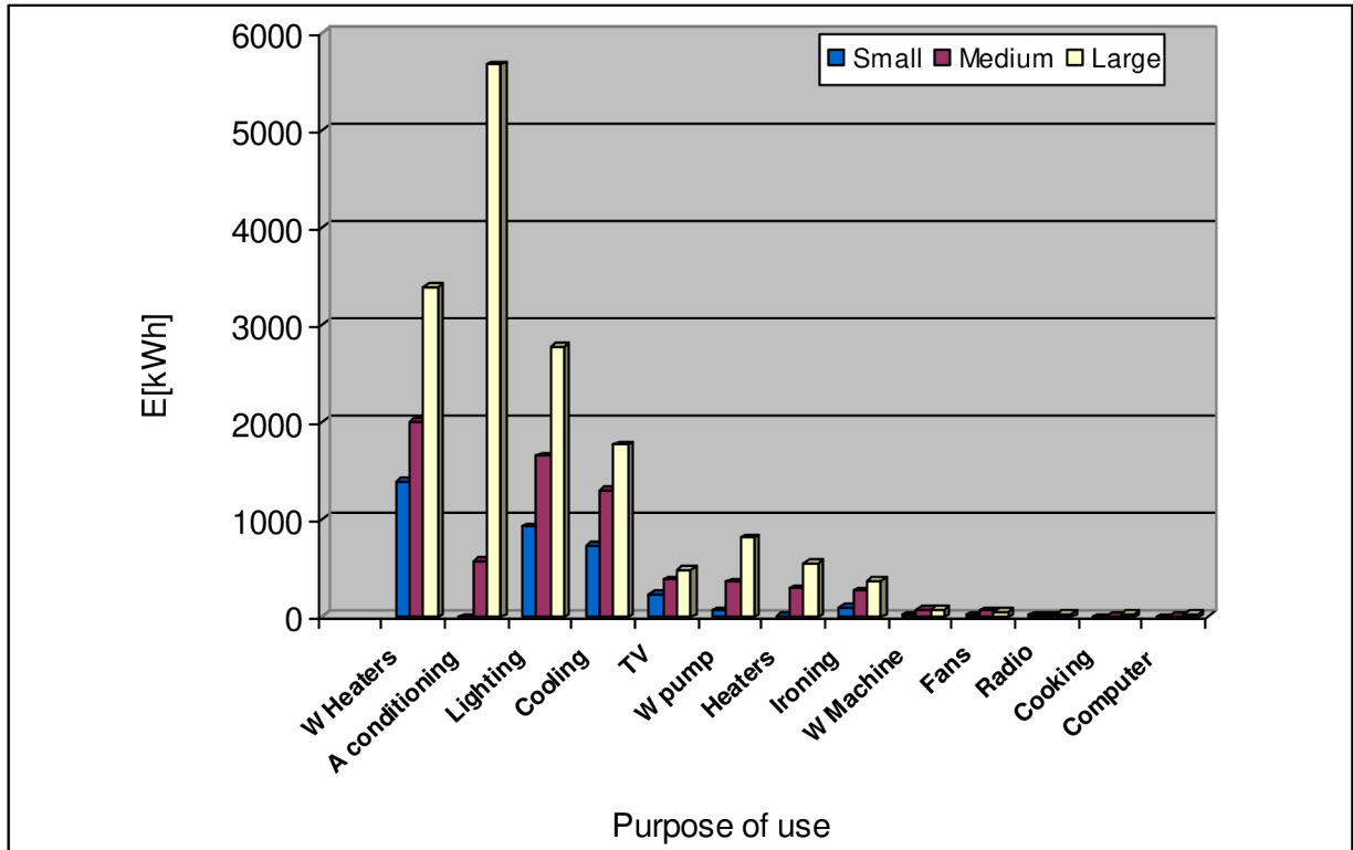
Fig. 11.2 Annual electrical energy consumption, depending of purpose of use, Tripoli
