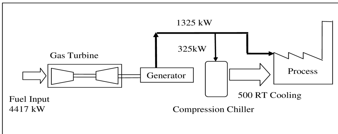
Fig. 9.6 Schematic diagram of power generation and cooling with electricity [39]
