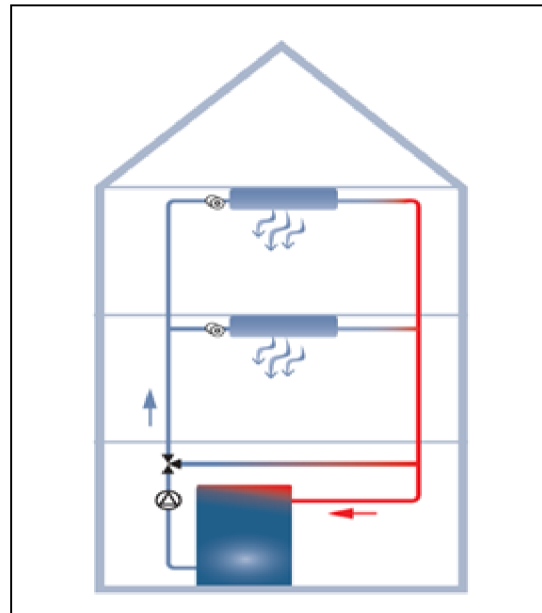
Fig. 11.11 Chiller system
