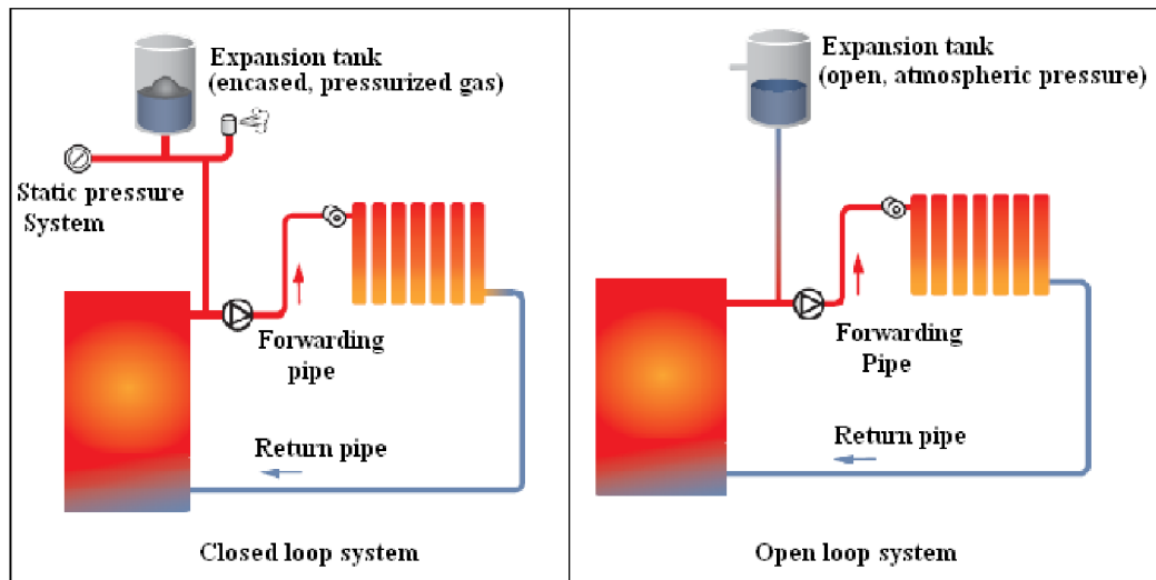
Fig. 11.8 Closed and Open loop systems [43]
