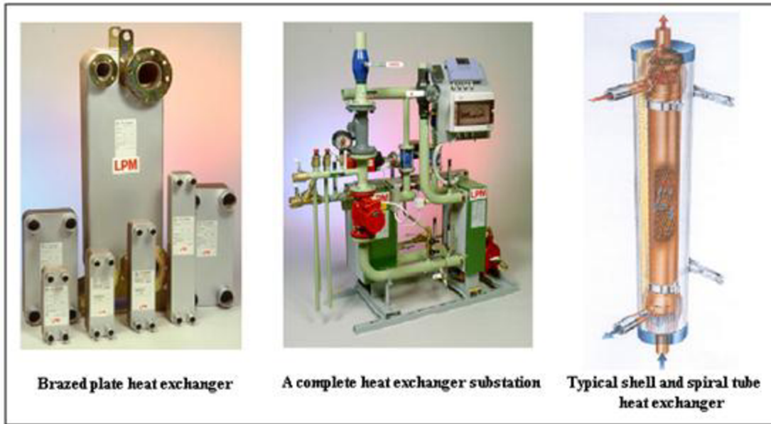
Fig. 11.7 Types of heat exchanger [42]
