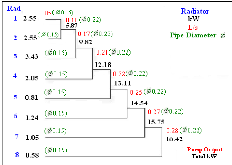
Fig. 11.16 Power flow in the system of small house network
