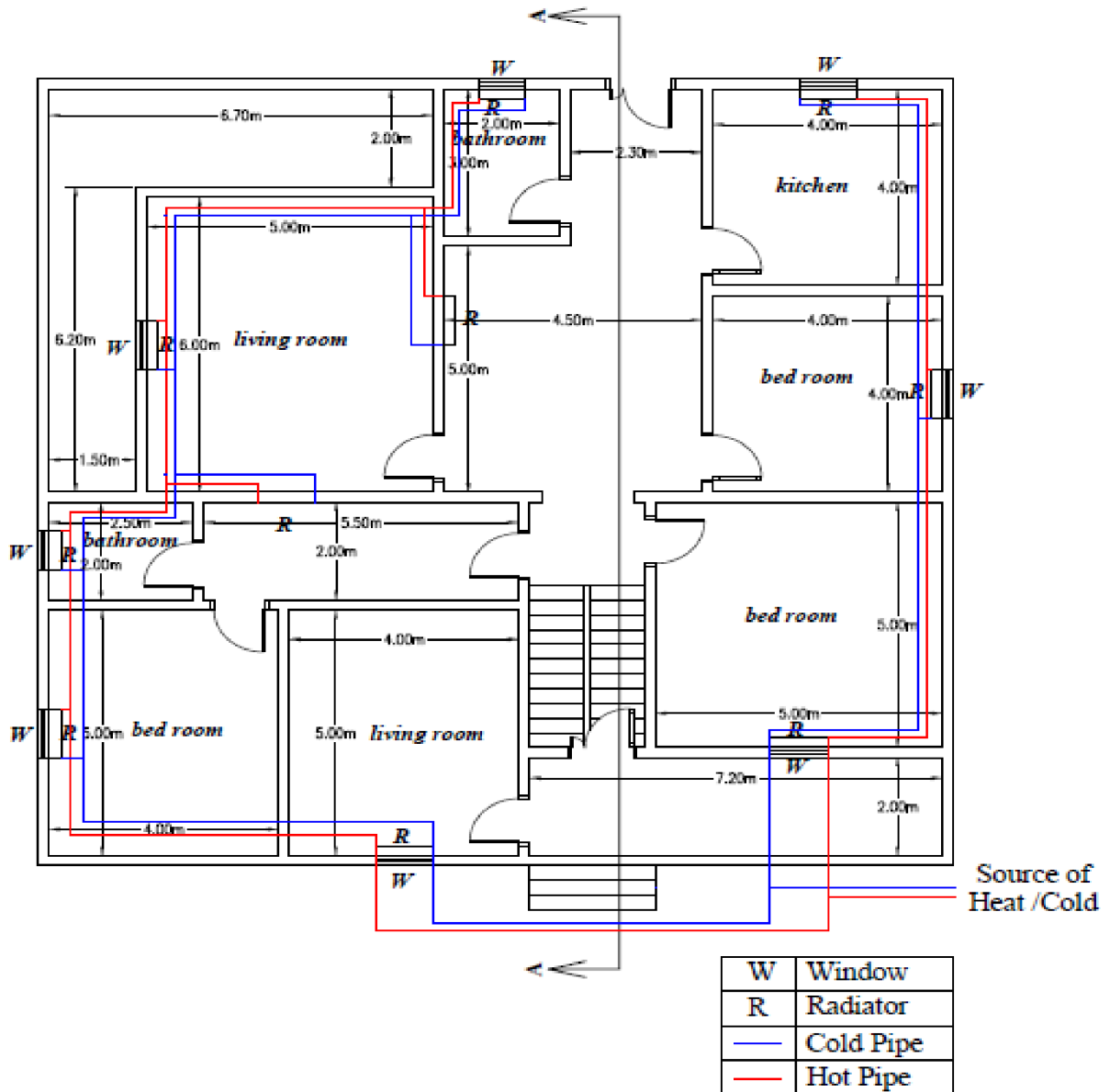
Fig. 11.23 Scheme for large house ground floor
