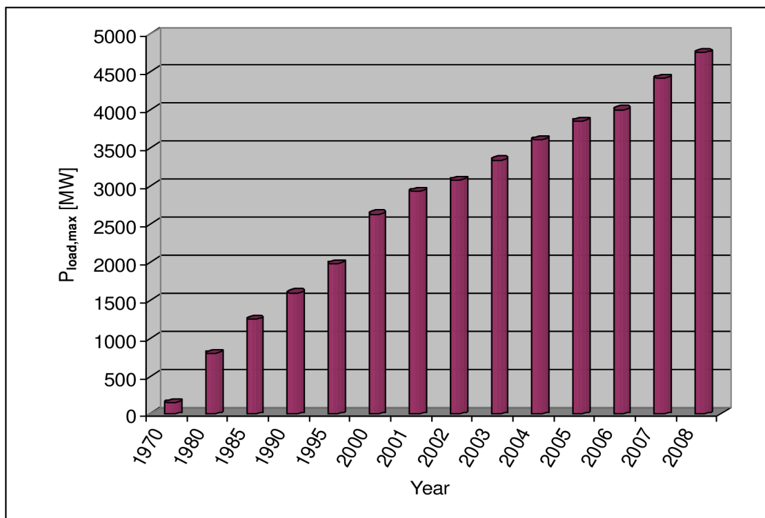
Fig. 4.10 Increasing of maximum load (1970-2008)
