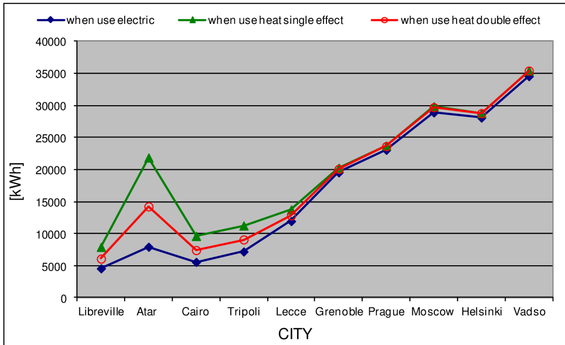
Fig. 12.3 Energy input (requirement) when use electrical & heat (single, double)
