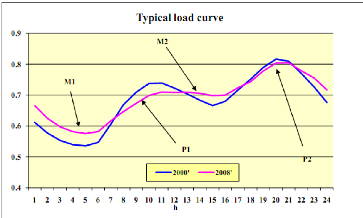
Fig. 4.17 Typical normalized daily Load curves for years 2000 & 2008. The normalization factor is the peak load within the respective year [15]
