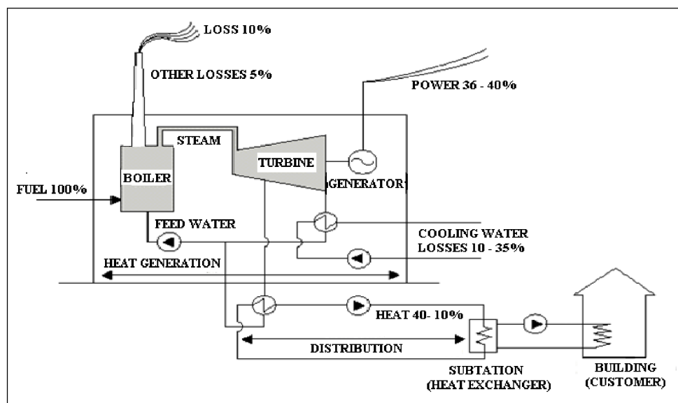
Fig. 10.1 District heating network [31]
