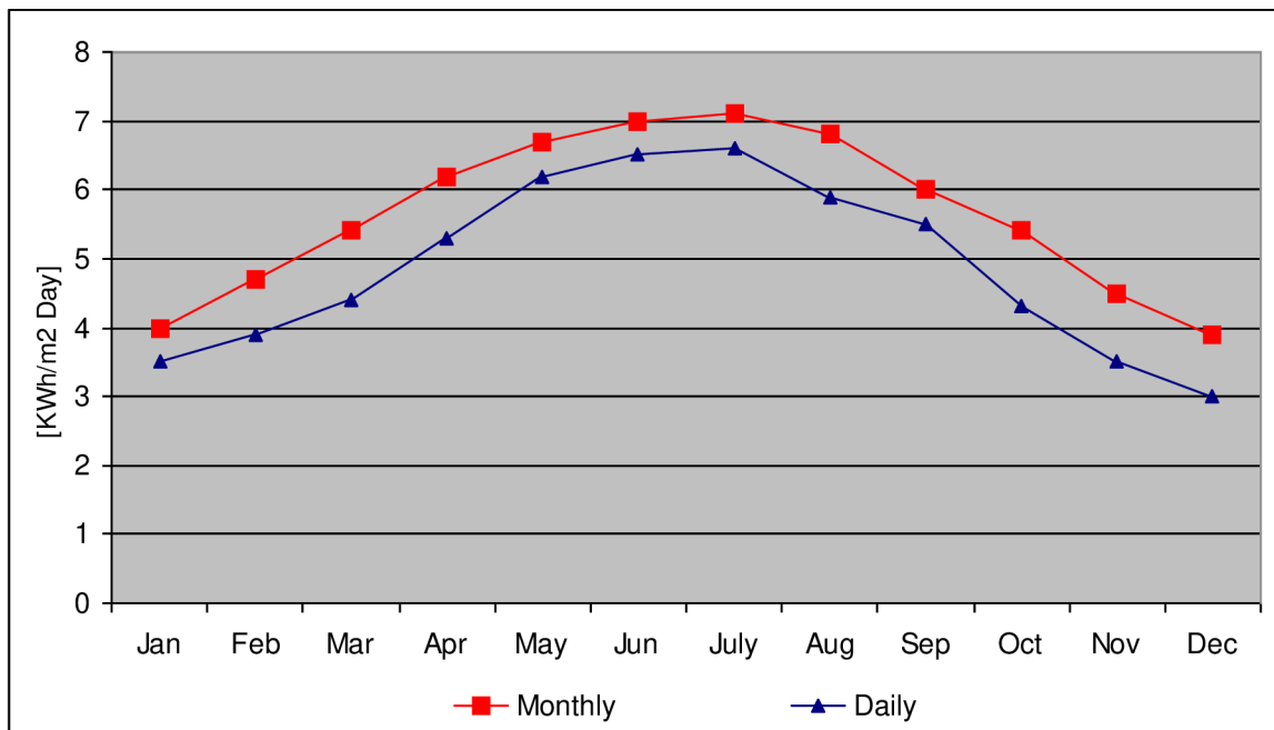
Fig. 4.1 Average monthly, daily solar radiation on horizontal surface [11]
