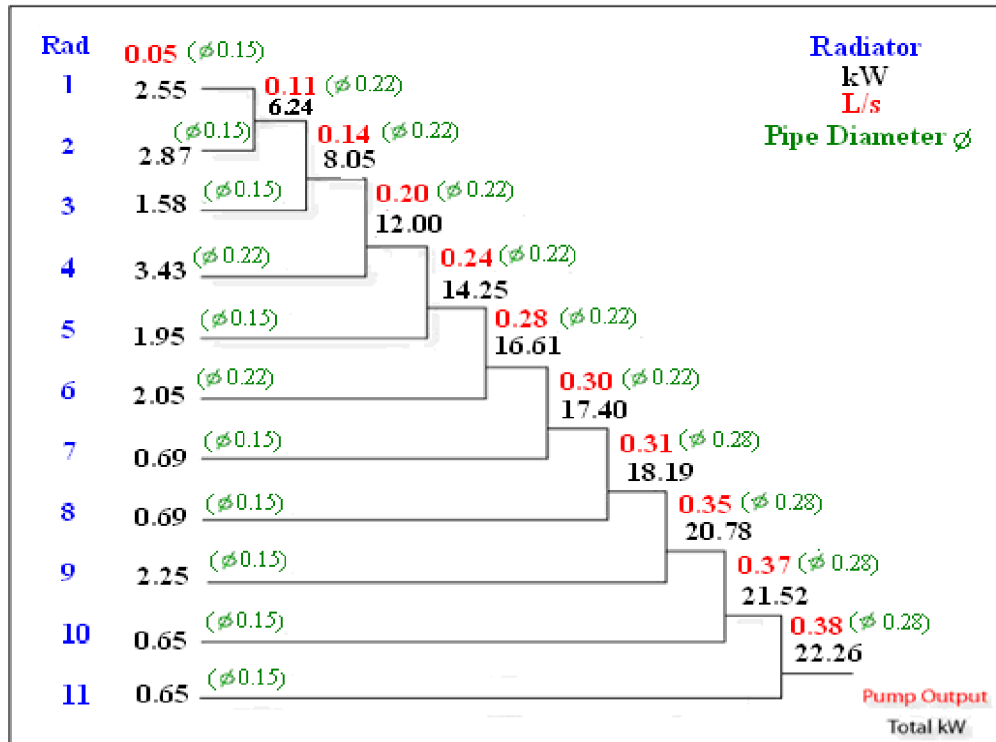
Fig. 11.21 Power flow in the system of medium house
