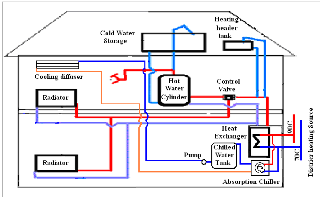
Fig. 11.6 Heating /cooling system for typical house
