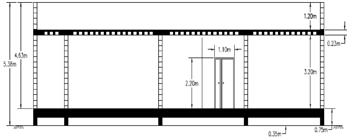
Fig. 11.19 Cross section A-A of the building
