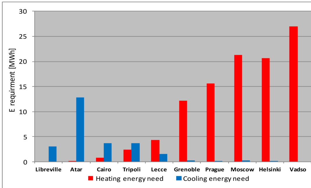
Fig. 12.2 Energy requirement for heating and cooling
