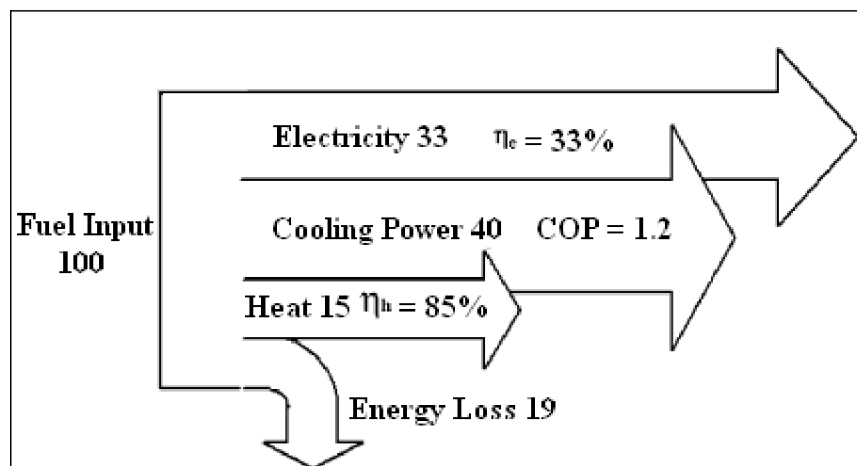
Fig. 9.9 Energy flow of typical CHCP system [27]
