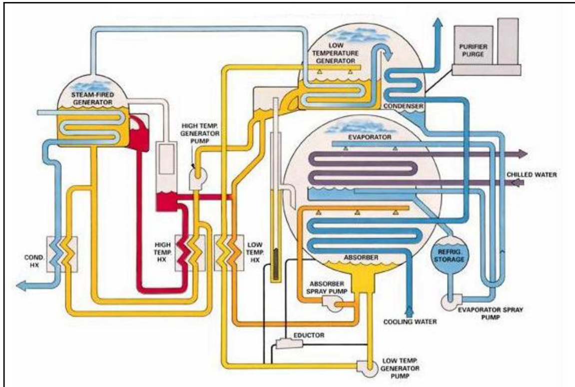
Fig. 9.5 Two stage-fired absorption machine
