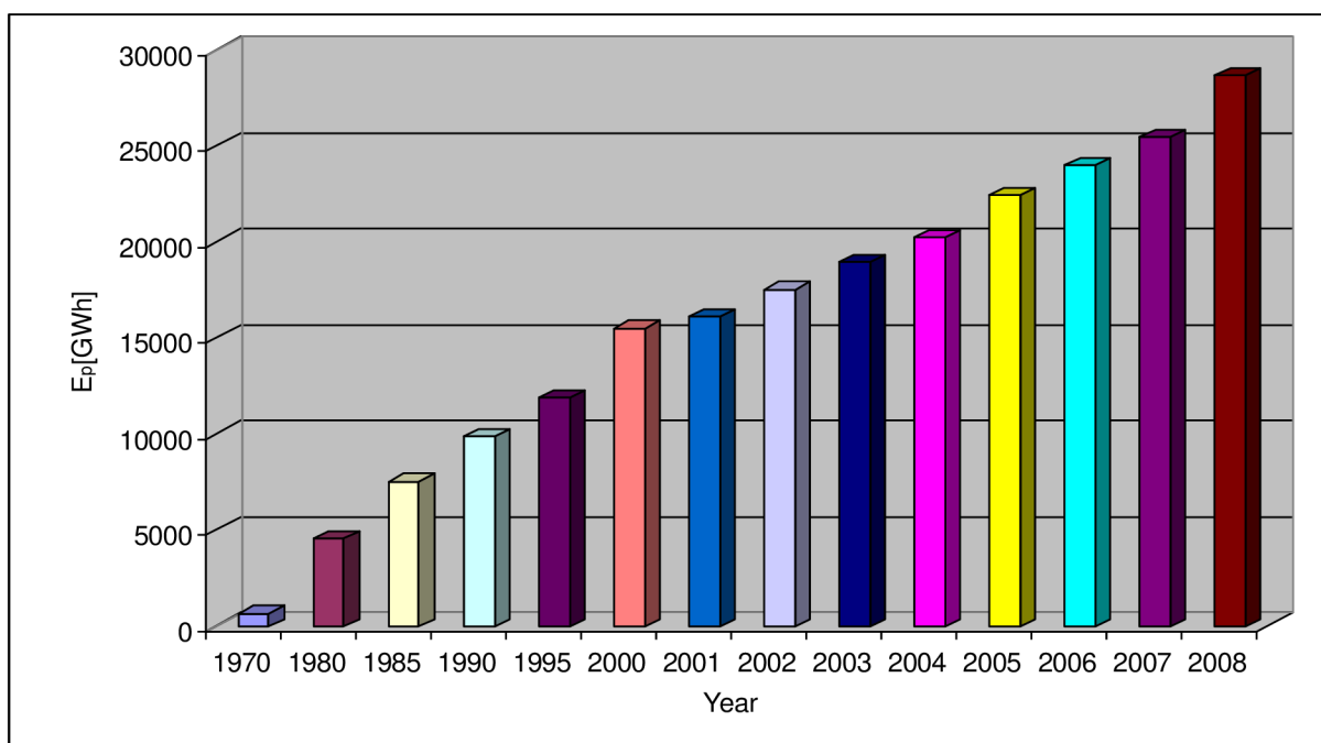
Fig. 4.8 Electrical energy production (1970-2008)
