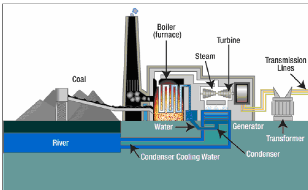
Fig. 7.1 Coal Fired Thermal Power Plant [60]
