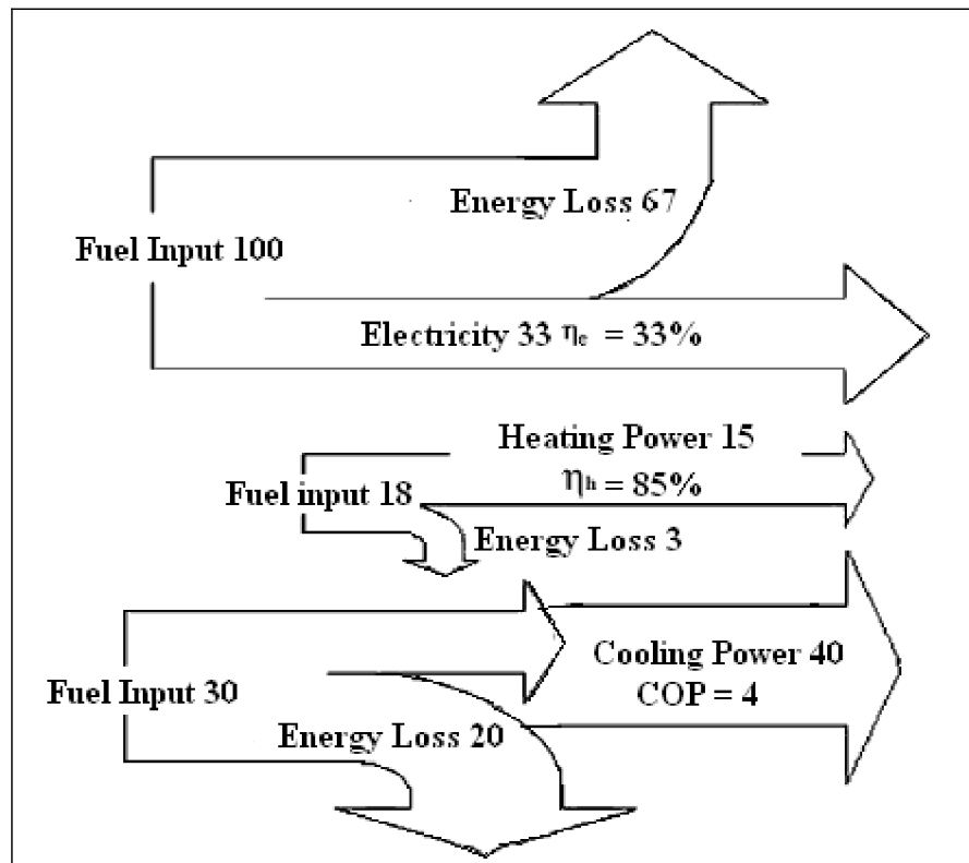
Fig. 9.8 Energy flow of traditional supply mode [27]
