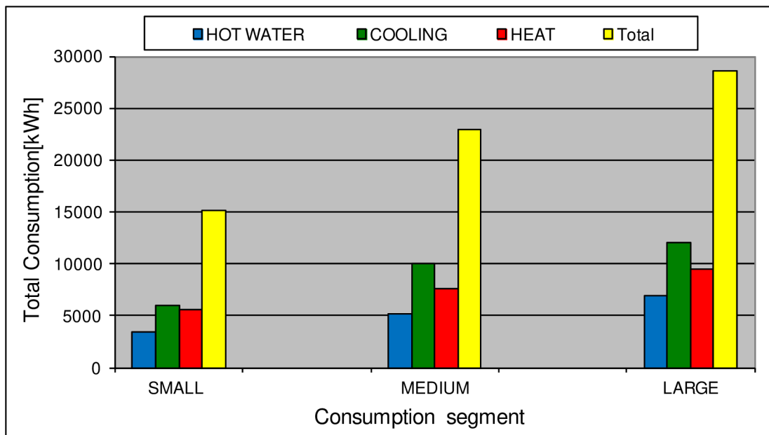
Fig. 11.29 Total consumption of energy
