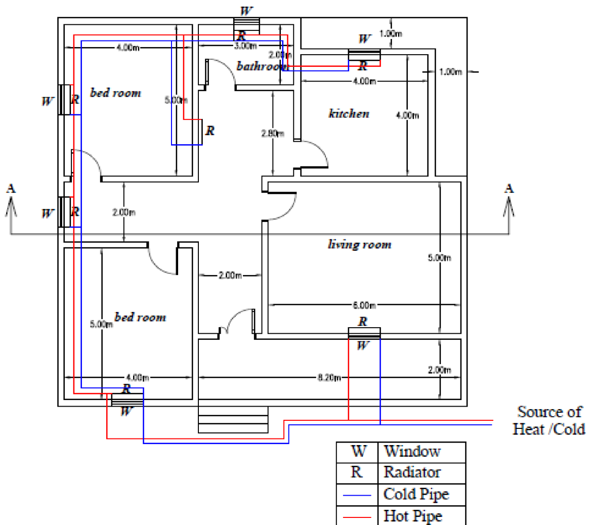
Fig. 11.13 Scheme for small house (Horizontal view)
