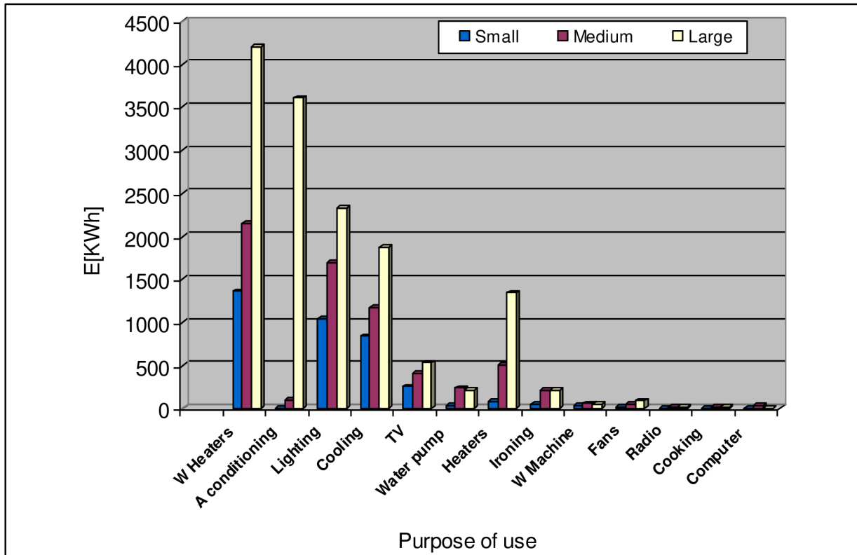
Fig. 11.3 Annual electrical energy consumption, depending of purpose of use, Benghazi
