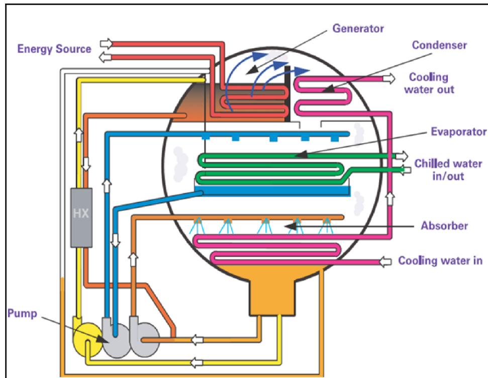
Fig. 9.4 The principal of an absorption cooling machine
