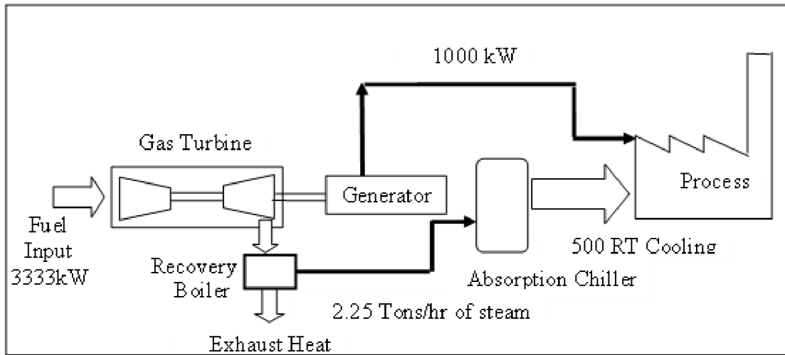
Fig. 9.7 Schematic diagram of power generation and absorption cooling [39]
