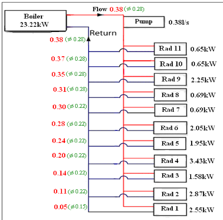
Fig. 11.22 Heating system of medium house
