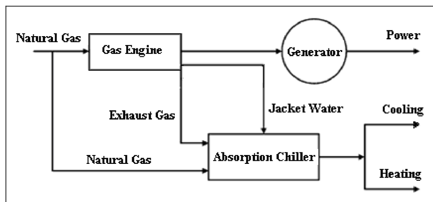
Fig. 9.3 Typical CHCP system [27]
