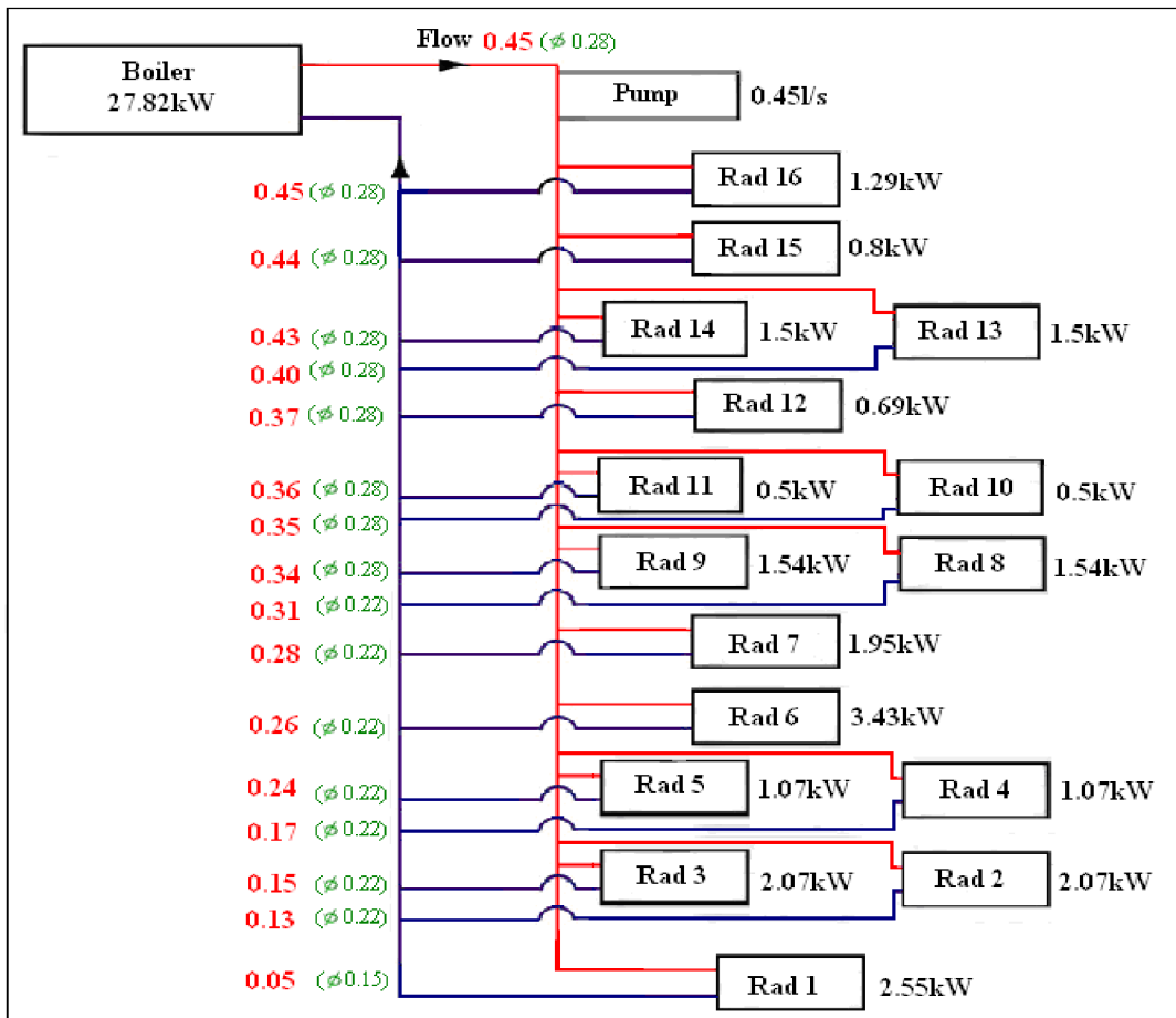
Fig. 11.28 Heating system of large house
