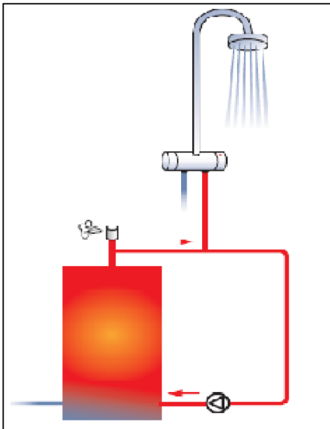
Fig. 11.10 Hot water system
