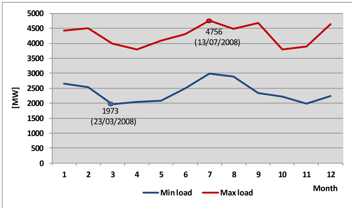
Fig. 4.18 Maximum and minimum load in 2008
