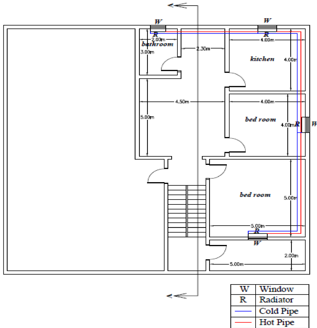
Fig. 11.24 Scheme of Large House first floor
