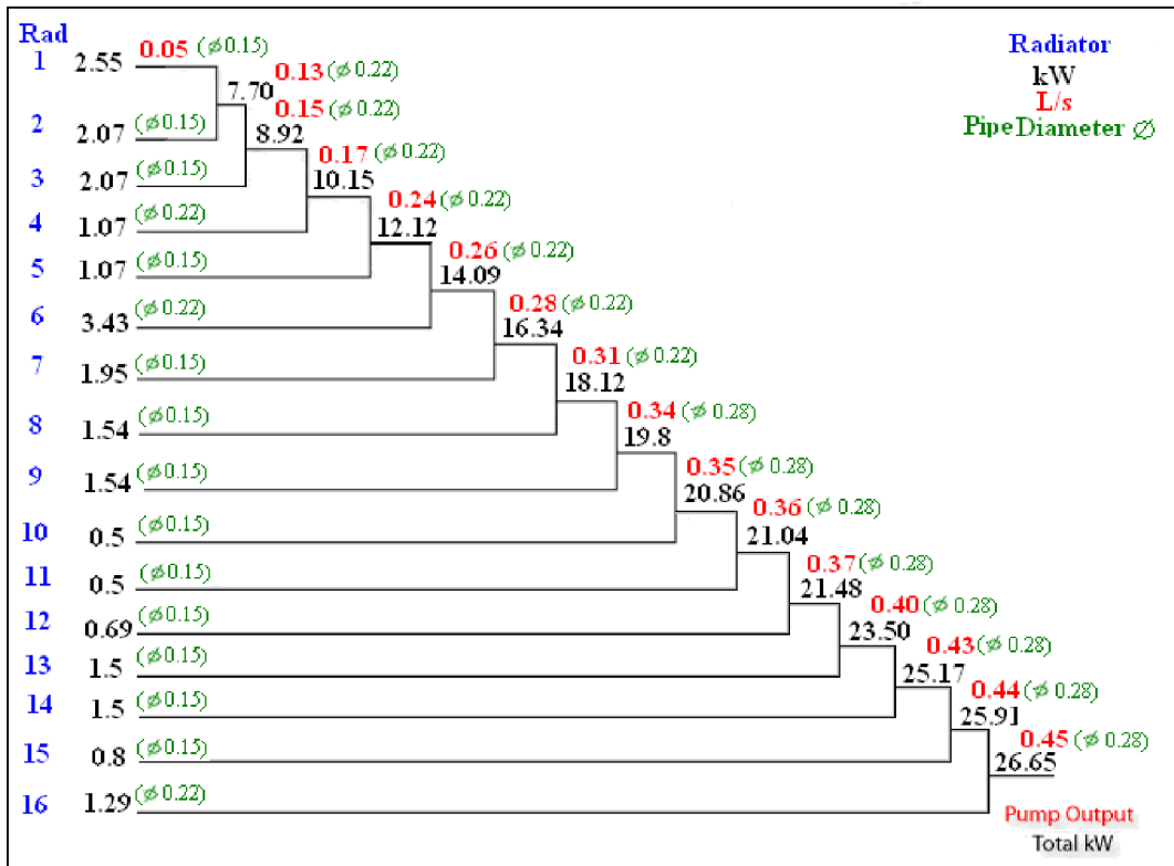
Fig. 11.27 Power flow in the system of large house network
