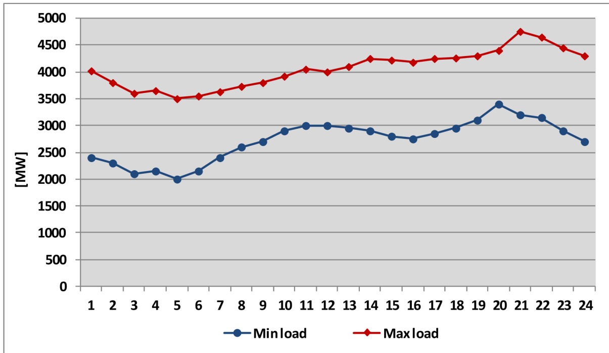
Fig. 4.19 Daily load curve of the maximum and minimum load in 2008
