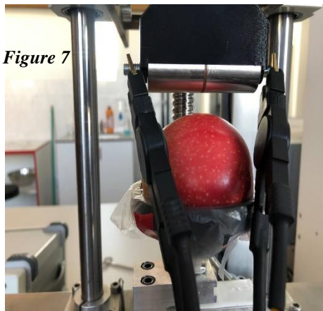
Figure 4, 5, 6, and 7: Process of capacitance measurements set up
