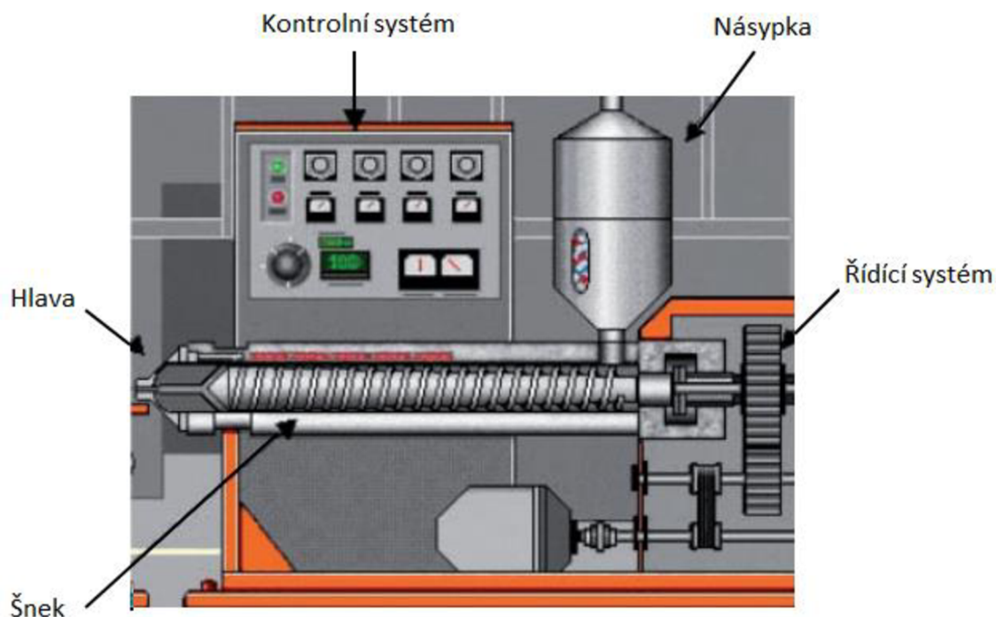
Obr. 3: Schéma extruderu [1]
