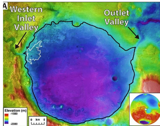
Figure 3.1: Jezero crater paleolake. Overview of the paleolake basin (centered at \sim 18.4^\circ\text{N} , 77.7^\circ\text{E} ). Black outline indicates the minimum basin breach level. White outline indicates the western delta deposit (Goudge et al., 2018).
