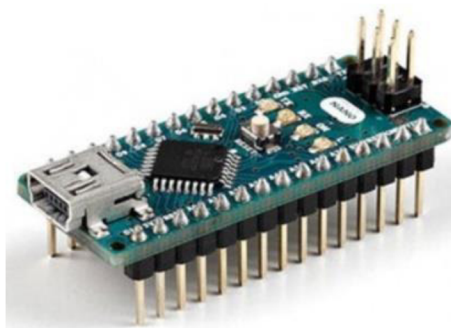
Obr. 4 Arduino Nano [3]
