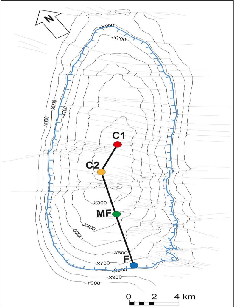
Figure 6: Contour map showing the depth of top of A0 in Field A. Blue line shows the oil-water contact (OWC) at the top of Thamama Zone A. Grey lines show the seismic picked faults. Circles in red, yellow, green, and blue show the location of the four studied wells in the crest (C1 and C2) and flanks (MF, F). (M. Alsuwaidi et al., 2022).
