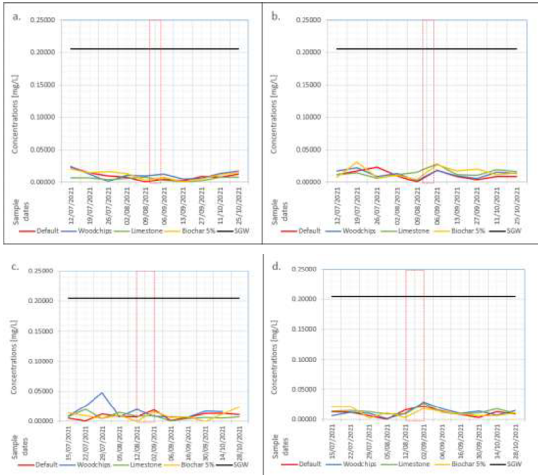
Figure 15. Cu removal efficiency after application of filtering materials during the experiment. A. 70-30% saturation after 72 hours. B. 30% saturation after 22 hours. C. 70-30% saturation at 22 hours. D. 30% saturation at 22 hours.
