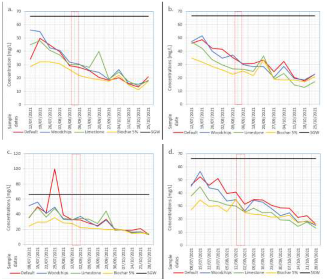
Figure: 8. Concentration of TOC after application of filtering materials during the experiment. A. 70-30% saturation after 72 hours. B. 30% saturation after 22 hours. Red timeframe indication. C. 70-30% saturation after 22 hours. D. 30% saturation after 22 hours.: 3 weeks break (12/08/2021-2/9/2021).
