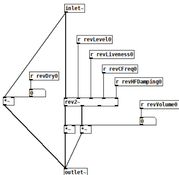
Obr. 4.31: Reverb
