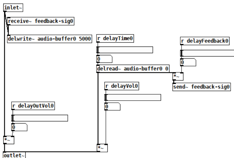
Obr. 4.30: Subpatch delay
