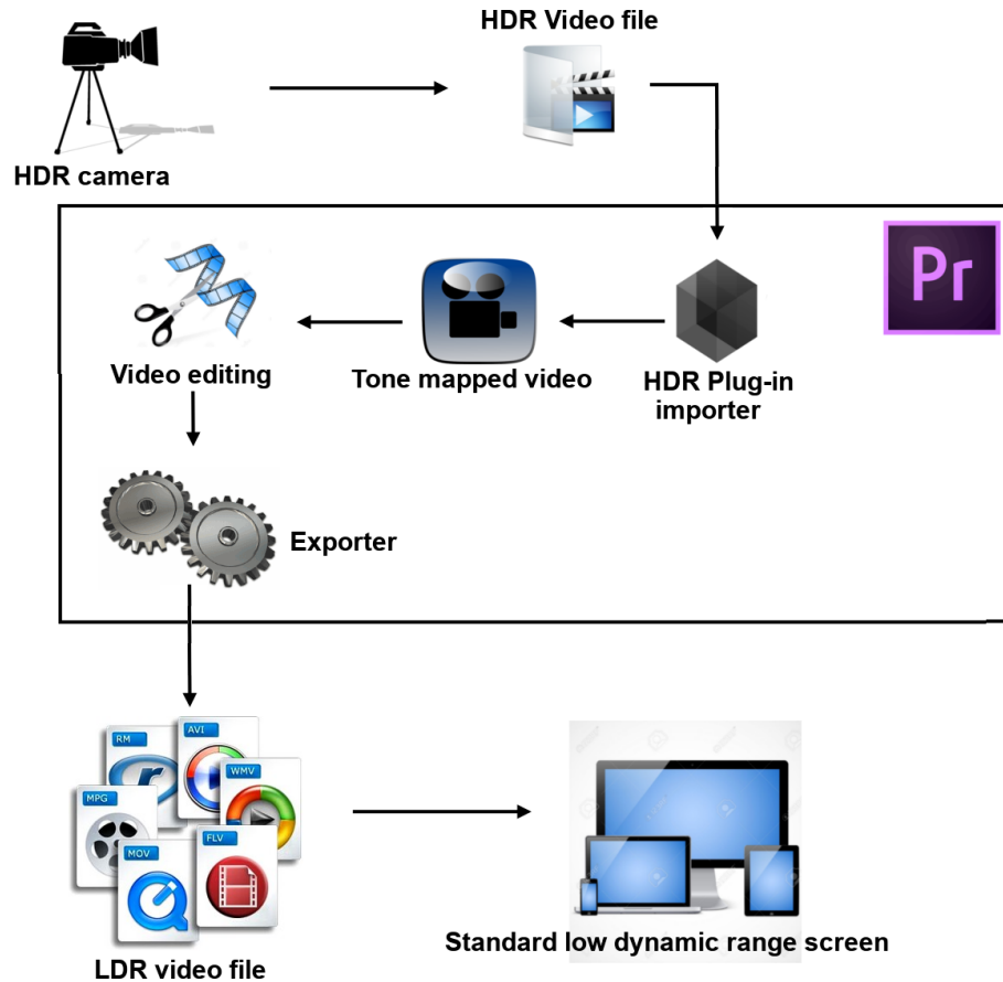
Figure 4.1: Workflow of video processing by HDR plug-in.
