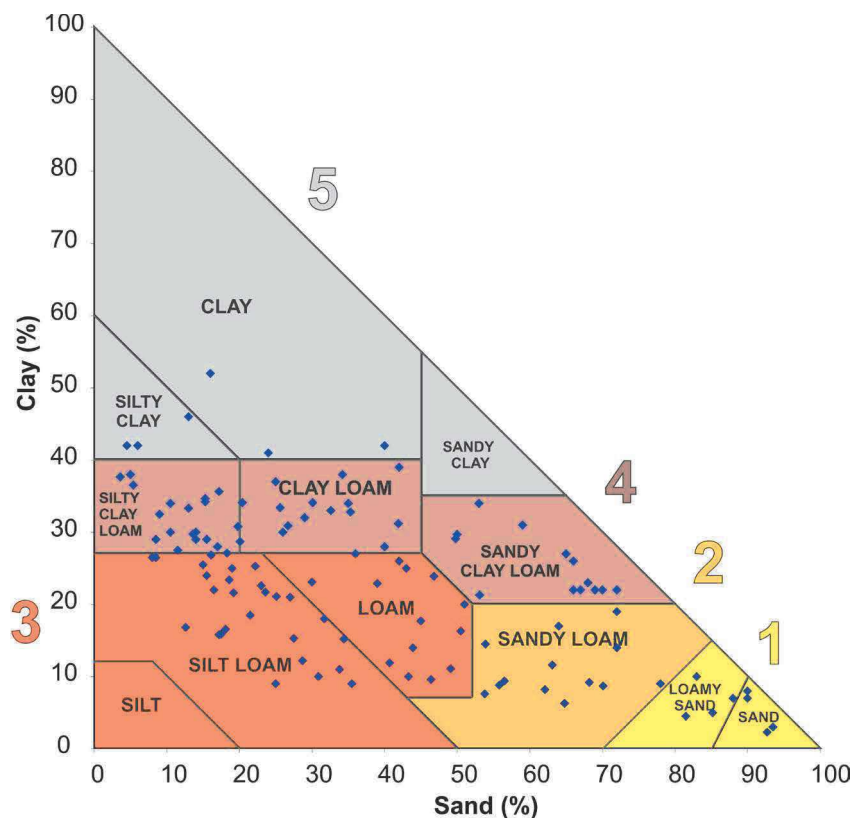
Figure 2. Particle size distribution data of soils used in this study within the USDA soil texture triangle, with coloured indications of the five grouped texture classes (from 1 to 5) according to Němeček et al. (2001)
