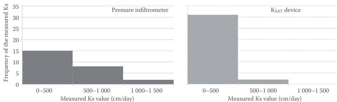
Figure 1. Frequency histograms of the measured saturated hydraulic conductivity (Ks) data; in-situ measurements utilising a Pressure infiltrometer by Matula and Kozáková (1997) on the left and laboratory measurements on 250 \text{cm}^3 undisturbed soil samples by a K_{SAT} device (METER Group Inc.) on the right
