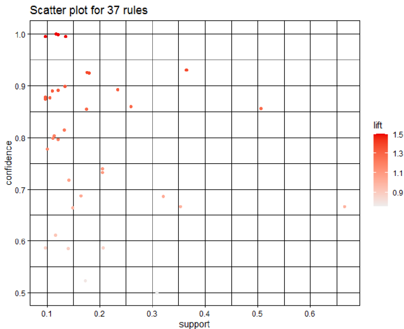
Figure 27: Association Rules 1 Source: Own contribution
