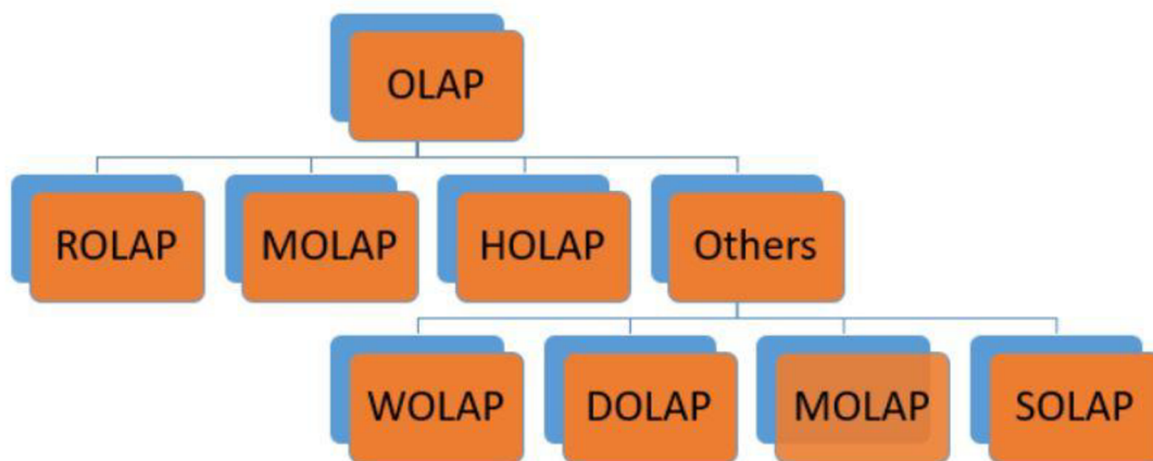
Figure 7: OLAP
