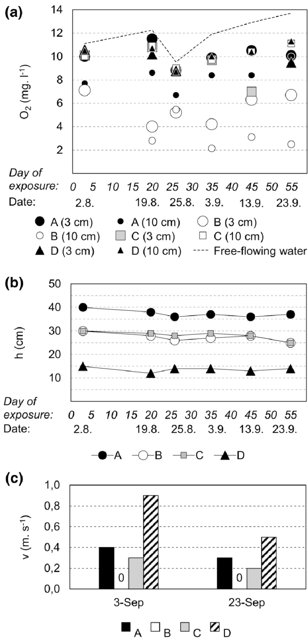
Fig. 4 Oxygen concentration changes ( \text{mg l}^{-1} ) in free-flowing water and sediment depths 3/10 cm (a), free-flowing water level depth changes (cm) (b) and flow velocity ( \text{m s}^{-1} ) 5 cm above the riverbed (c) at four sites A–D during the main experiment (Aug–Sep 2015). a Free-flowing water: dashed black line; site A (3/10 cm): large/small black circle, site B (3/10 cm): large/small white circle, site C (3/10 cm): grey/white square, site D (3/10 cm): large/small black triangle. b Site A/B/C/D: black circle/white circle/grey square/black triangle. c Site A/B/C/D: black/white/grey/black and white bar
