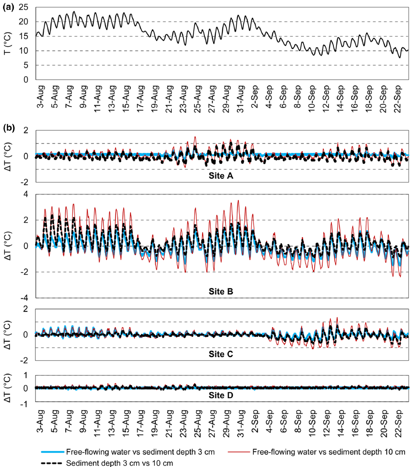
Fig. 5 Temperature changes ( ^{\circ}\text{C} ) in free-flowing water (a), and temperature differences between free-flowing water and sediment depths 3/10 cm at four sites A–D (b) during the main experiment (AUG–SEP 2015). b Free-flowing water vs
