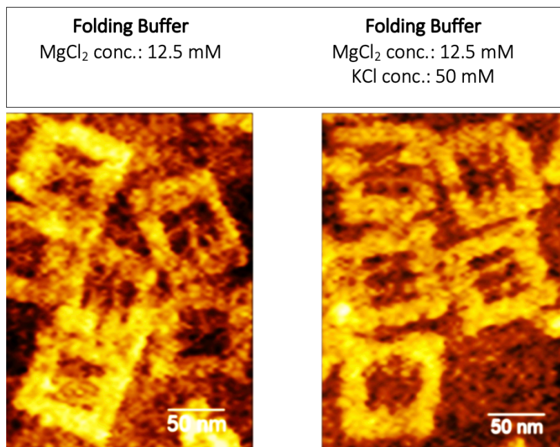
Figure 4.23: AFM images of DNA origami frames with incorporated GQs, deposition on Si substrate with folding buffer containing 12.5 mM Mg 2+ cations (left) and with folding buffer containing 50 mM K + cations (right) [author].
