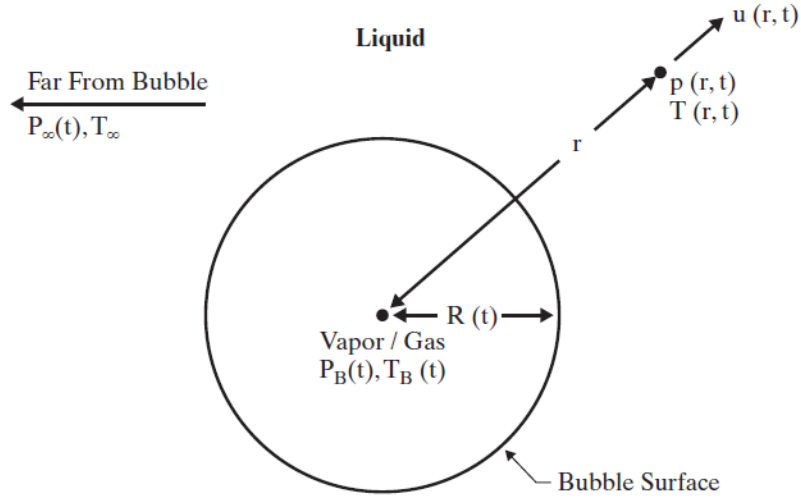
Figure 2.1 Schematic of a spherical bubble in an infinite liquid [2]
