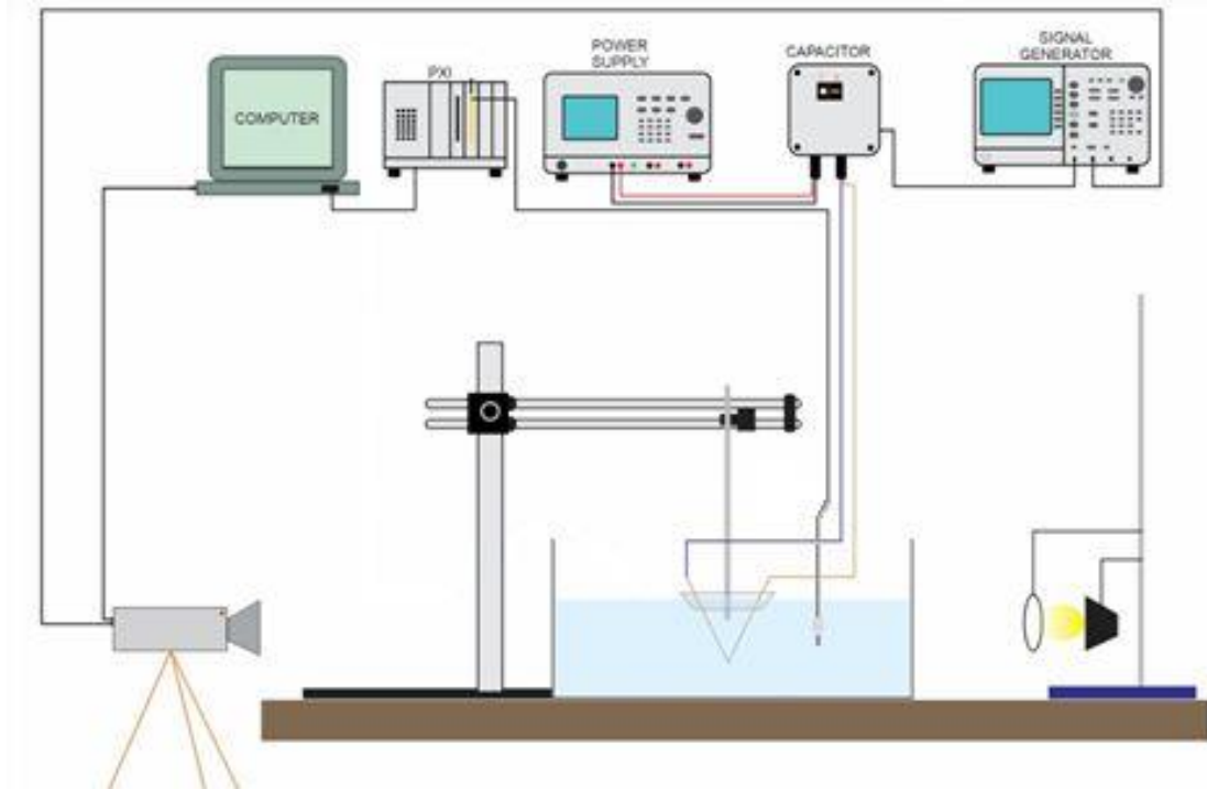
Figure 3.12 Experimental setup for spark-generated bubble
