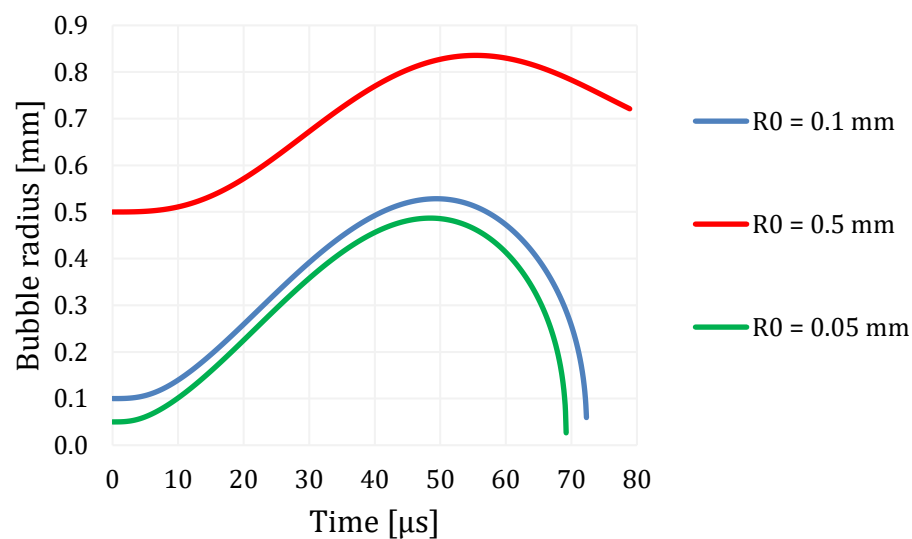
Figure 3.3 Influence of initial bubble radius on overall bubble growth
