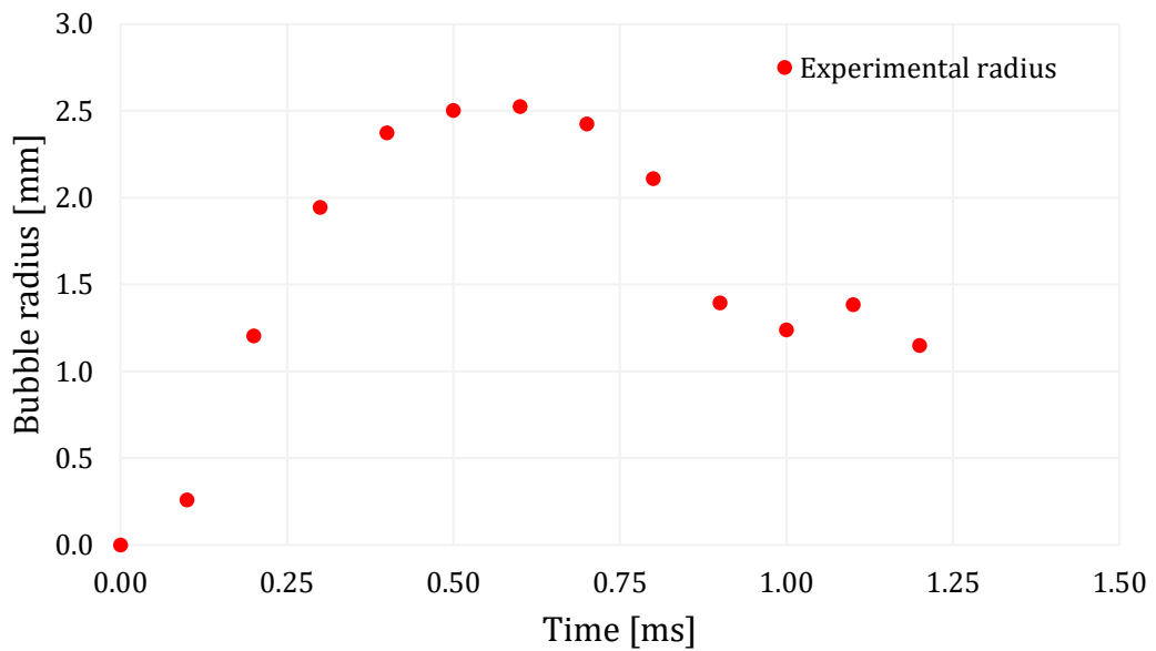
Figure 3.16 Radii obtained by the experiment - second spark-generated bubble
