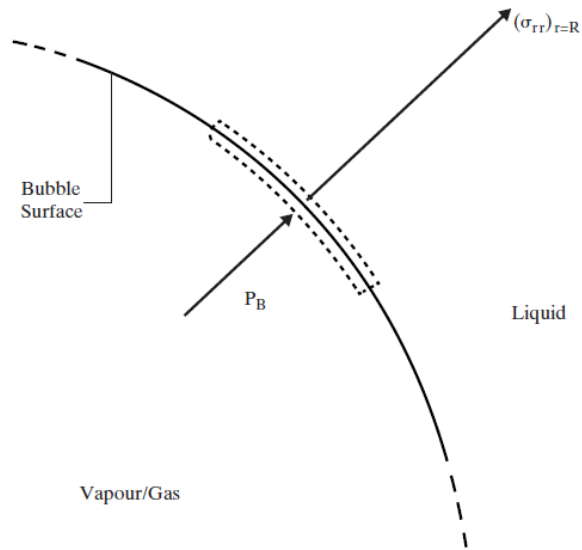
Figure 2.2 Lamina on the spherical bubble surface [2]
