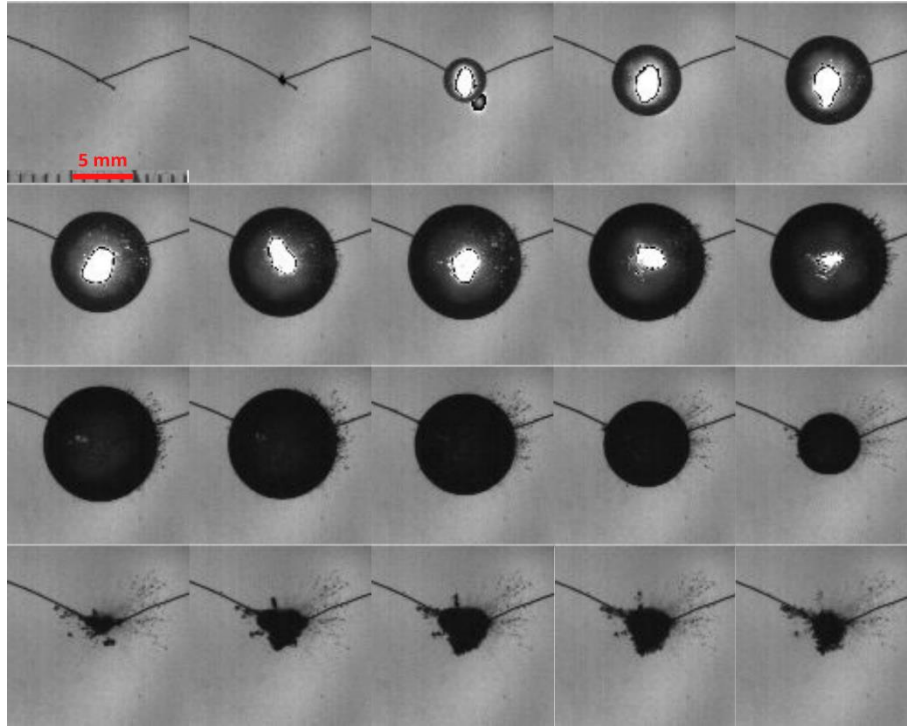
Figure 3.13 Visualisation of first two cavitation bubble collapses – first spark-generated bubble (time between each frame is 100 \mu\text{s} )
