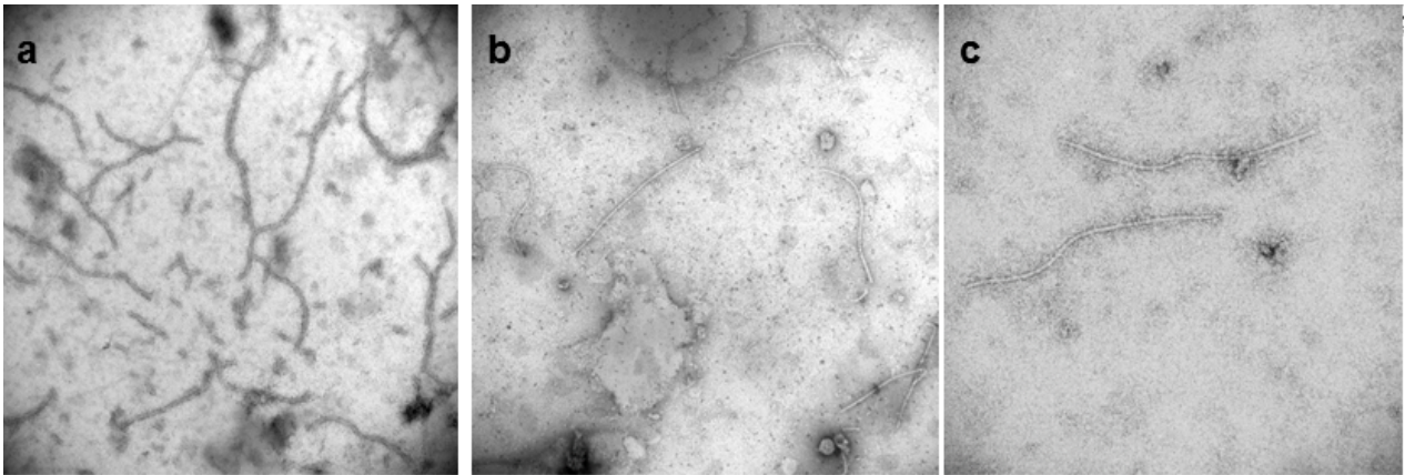
Figure 1 Transmission electron microscopy showing particles of Alexivirus from garlic plants. a: Dip preparation (negative staining with 1 % uranyl acetate), b: Immunosorbent electron microscopy and decoration (ISEM+DECO) of GarV-B, c: ISEM+DECO of GarV-D. (© Julius-Kühn-Institut, Braunschweig).
