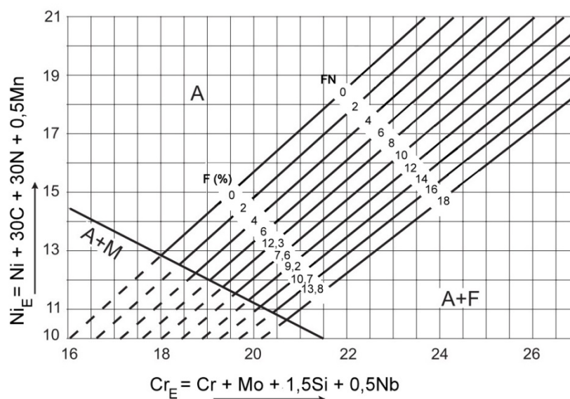
Obr. 4. 3: De Longüv diagram [27]
