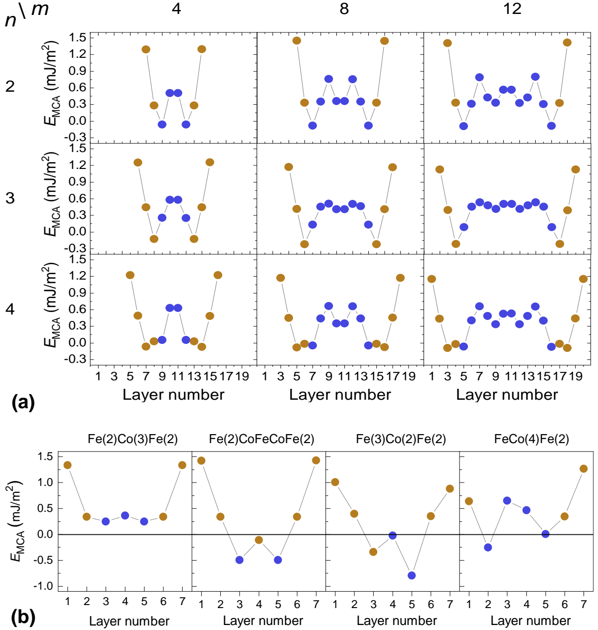
Figure 4.2: (a) Layer-resolved E_{MCA} in structures of the form \text{Fe}(n)/\text{Co}(m)/\text{Fe}(n)|\text{MgO} . Gold circles represent Fe layers and blue circles represent Co layers. The enhancement of E_{MCA} compared to a pure \text{Fe}|\text{MgO} structure is provided by the bulk Co layers, similar to Fig. 4.1 [120]. The Fe/Co interface is detrimental to the bulk Co PMA of the Co layer closest to Fe. (b) We find that at least 2 Fe layers and 3 Co layers are needed for the enhancement. This "minimal" structure is on the very left. The other structures defying this condition do not exhibit the large enhancement. © 2021 American Physical Society [120].
