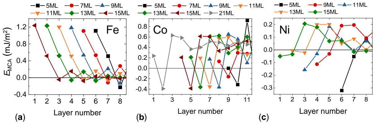
Figure A.1: Layer-resolved E_{MCA} for different thicknesses of (a) Fe, (b) Co, and (Ni) on MgO. © 2021 American Physical Society [120].
