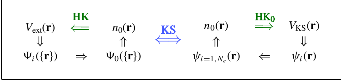
Figure 2.4: The KS mapping of the real problem onto one-electron problem. The left half corresponds to Fig. 2.3. Adapted from [37].
