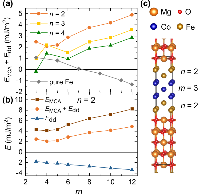
Figure 4.4: (a) Effective PMA ( E_{\text{MCA}} + E_{\text{dd}} ) in \text{MgO}|\text{Fe}(n)\text{Co}(m)\text{Fe}(n)|\text{MgO} as a function of number of monolayers n , m . There is no perpendicular to in-plane magnetic anisotropy switching compared to pure \text{MgO}|\text{Fe}|\text{MgO} (grey diamonds; its thickness is m+4 ML, the same as the overall thickness for n=2 ) [120]. (b) E_{\text{MCA}} , E_{\text{dd}} , and the effective PMA ( E_{\text{MCA}} + E_{\text{dd}} ) for n=2 . The effective PMA increases with the Co thickness [120]. (c) Supercell of the \text{MgO}|\text{Fe}(2)\text{Co}(3)\text{Fe}(2)|\text{MgO} with periodic boundary conditions applied in all directions [120]. Produced by VESTA [131]. © 2021 American Physical Society [120].
