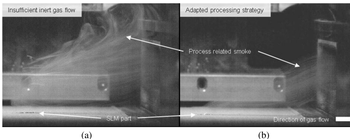
Fig 2.2 Recording of vapours during the AZ91D alloy printing process: (a) without modification of the inert atmosphere circuit; (b) with a modified inert atmosphere circuit [43].
