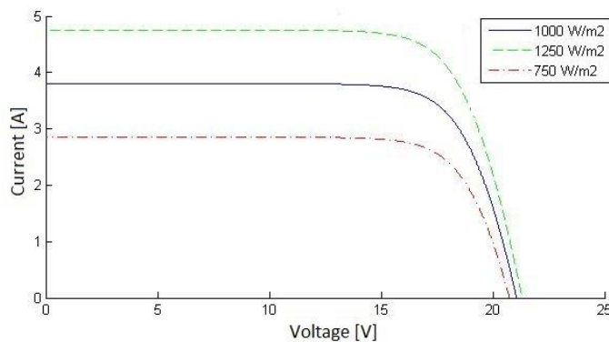
Figure 19: The effect of irradiance on the I-V curve of the PV module (Chaaban M. A., 2020).
