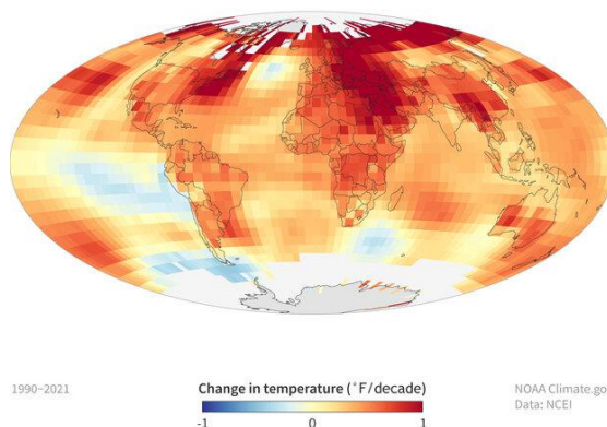
Figure 1: Change in global temperature from 1990 to 2021 (NOAA, 2021).
