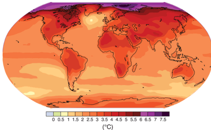
Figure 5: Increase in global temperature that is projected by 2099 (IPCC, 2021)
