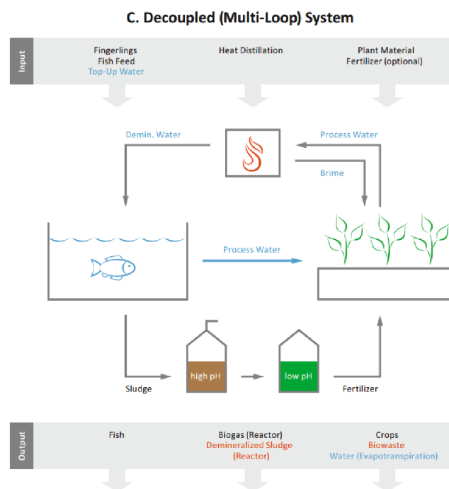
Fig. 25 Mechanism of a decoupled multi-loop aquaponic system [38] (for license details see page 93)
