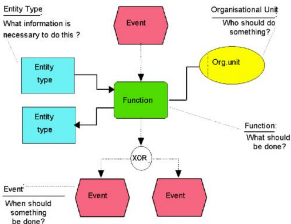
Figure 4: IDEF Diagram
