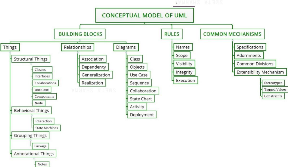
Figure 5: UML Model
