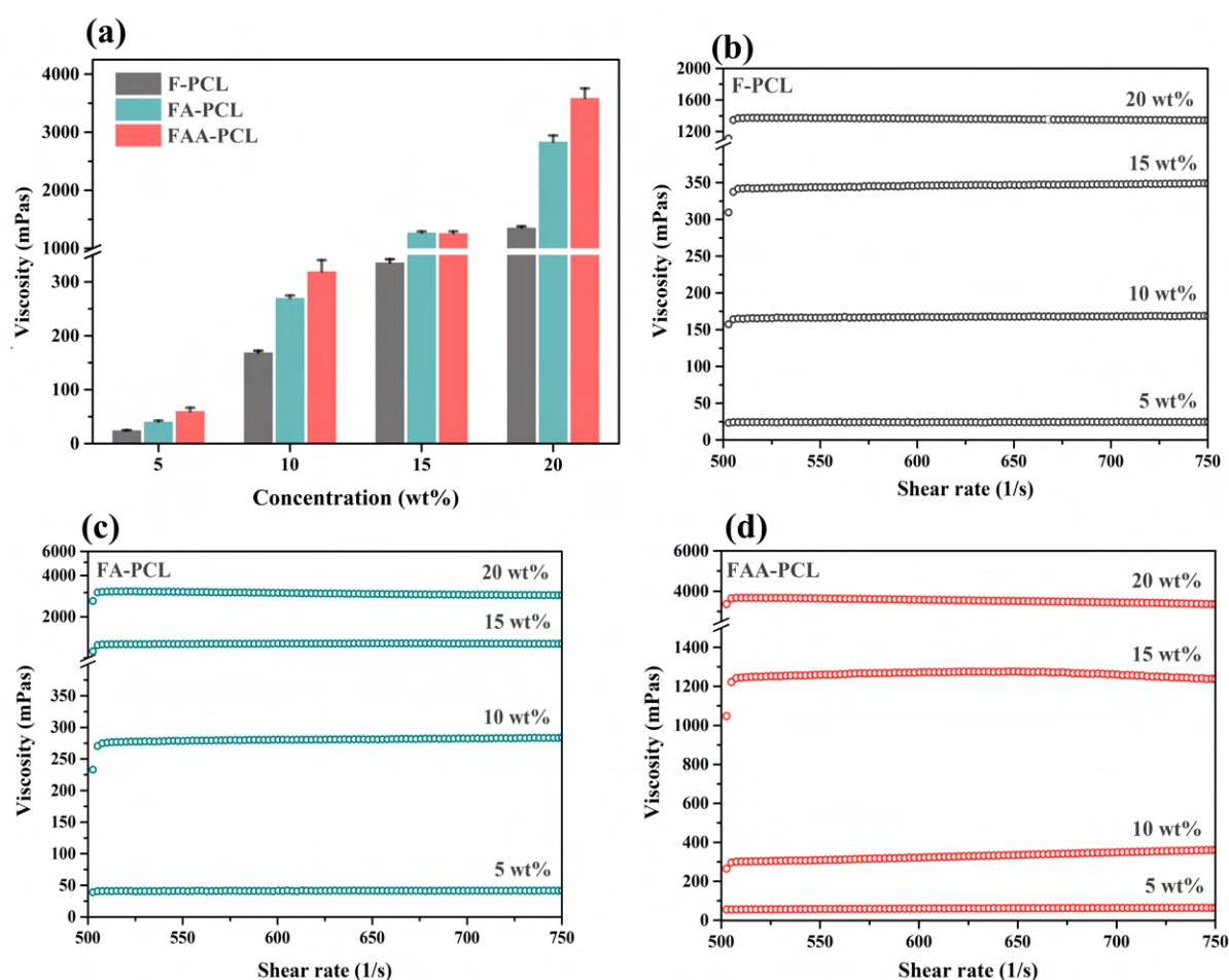
Figure 4.5: (a). The viscosity of FAA–PCL, FA–PCL, and F–PCL precursor solutions corresponding to precursor concentration and (b–d) the precursor solution viscosity as a function of shear rate (the dynamic viscosity values are shown in milli Pascal-second (mPas)).
