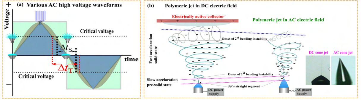
Figure 2.4: (a) Electrohydrodynamic instability and jet ejection as a function of the time and voltage for various waveforms ( \Delta t_S and \Delta t_T is the time interval between changes in the voltage polarity for the sine and triangle waveforms, respectively), and (b) The polymeric jet under the DC and AC electric field [61]
