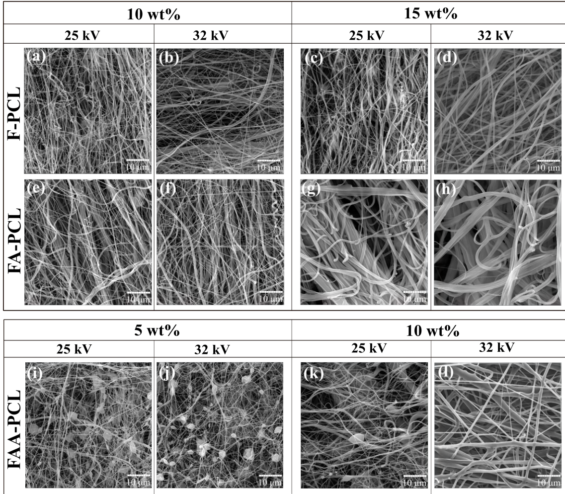
Figure 4.6: SEM micrographs of various PCL ENS as a function of the various solvent systems (F, FA, and FAA), polymer concentrations (5, 10, and 15 wt%), and applied high voltage (25 and 32 kV_{RMS} ).
