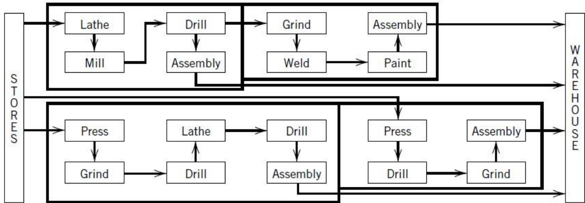
Figure 15: Product Family Layout[18]
