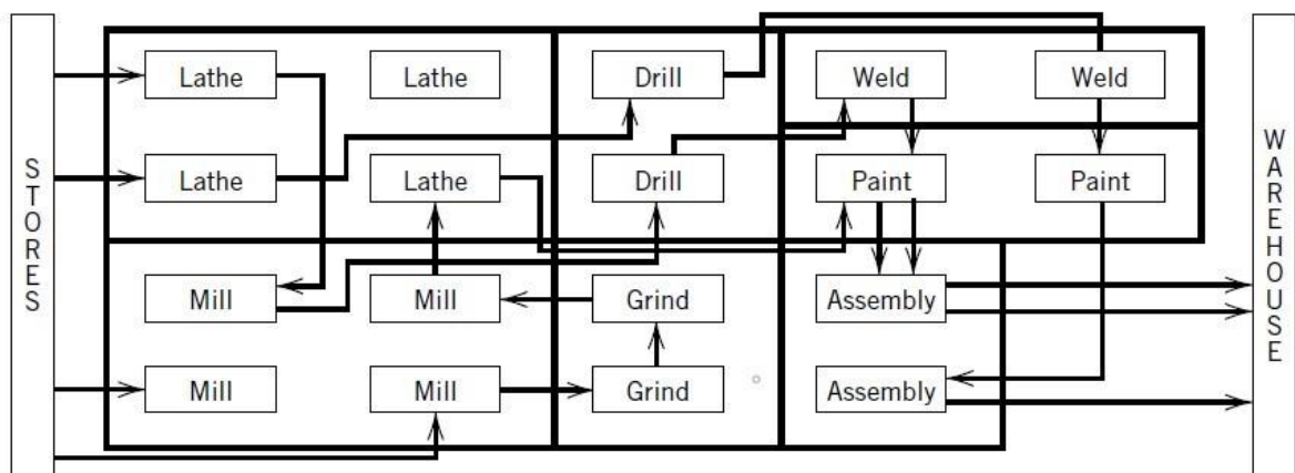
Figure 16: Process Layout[18]
