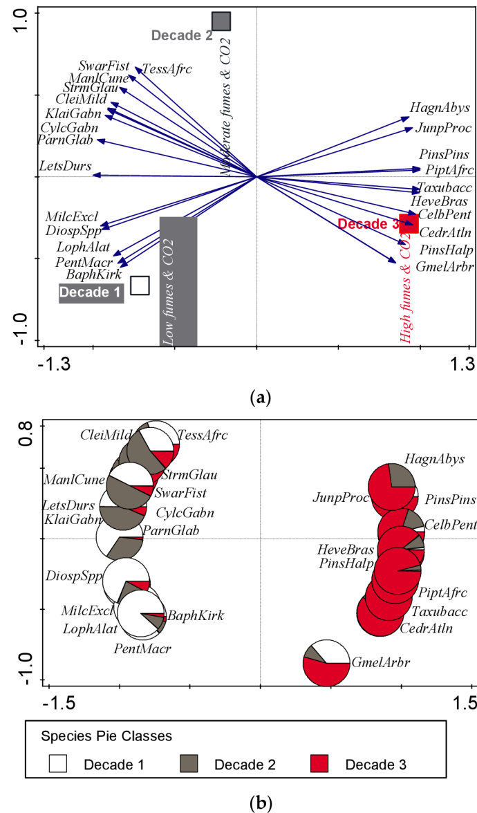
Figure 6. Biplot from the multivariate analysis of ordination showing the study decades and their associated common tree species for the wood charcoal production in the four countries (Nigeria, Ghana, Senegal and Ethiopia). (a) Indicated the distribution of species and their pollution emission (fumes and CO 2 ) status for each decade, (b) showed the proportion of species for each decade. Description of the plant species abbreviations is shown in Table 4.
