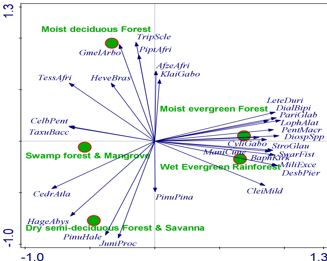
Figure 8. Multivariate ordination plot showing the vegetation zones and their associated common tree species, which promoted carbon fluxes vis-à-vis sustainable forest bioeconomy for each vegetation zone during the study period. Description of the abbreviations are as follows for each species: Dialium bipindense = DialBipi; Diospyros spp. = DiospSpp; Pentaclethra macrophlla = PentMacro; Letestua durissima = LeteDuri; Lophira alata = LophAlat; Milicia excels = MiliExce; Baphia kirkii = BaphKirk; Cleistanthus mildbraedii = CleiMild; Cylicodiscus gabonensis = CyliGabo; Desbordesia pierreana = DesbPier; Manilkara cuneifolia = ManiCune; Parinari glabra = PariGlab; Strombosia glaucescens = StroGlau; Swartzia fistuloides = SwarFist; Tessmania Africana = TessAfri; Klainedoxa gabonensis = KlaiGabo; Azelia africana spp = AfzeAfri; Piptadeniastrum africanum = PiptAfri; Triplochiton scleraxylon = TripScle; Gmelina arborea = GmelArbo; Juniperus procera = JuniProc; Pinus halepensis = PinuHale; Pinus pinaster = PinuPina; Cedrus atlantica = CedrAtla; Hagenia abyssinica = HageAbys; Taxus baccata = TaxuBacc; Hevea brasiliensis = HeveBras; Celba pentandra = CelbPent.
