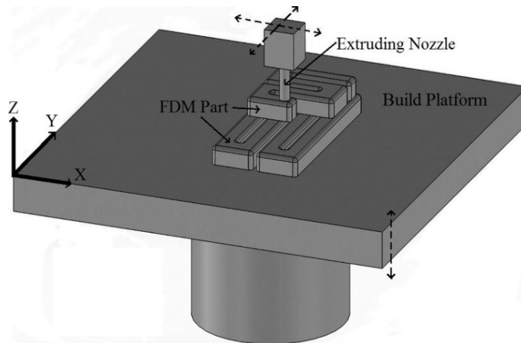
Obr. 10: Princip FDM [48]
