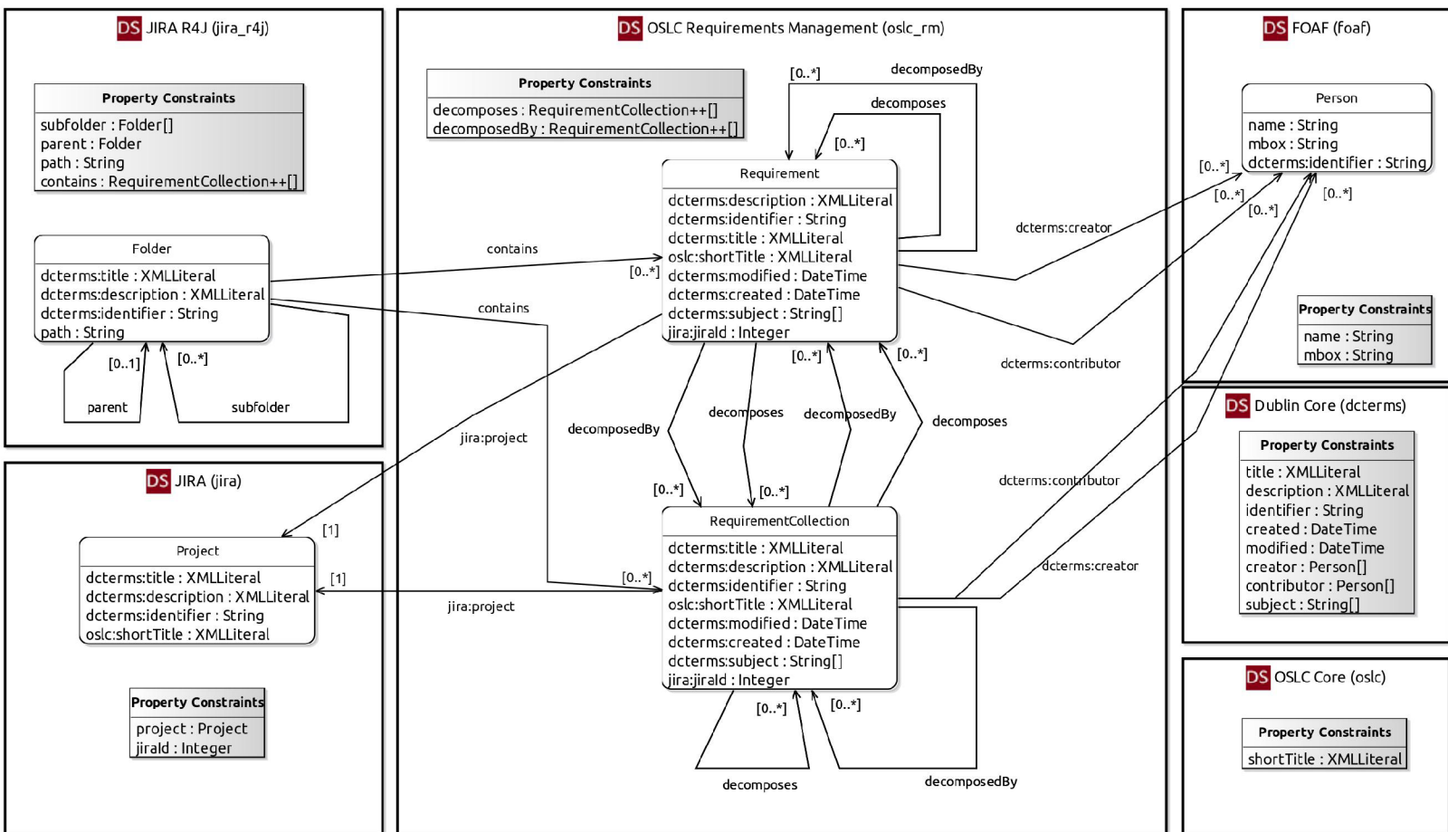
Figure 5.3: OSLC Requirement Management Domain Model Diagram (Exported from Ligo modeling tool)
