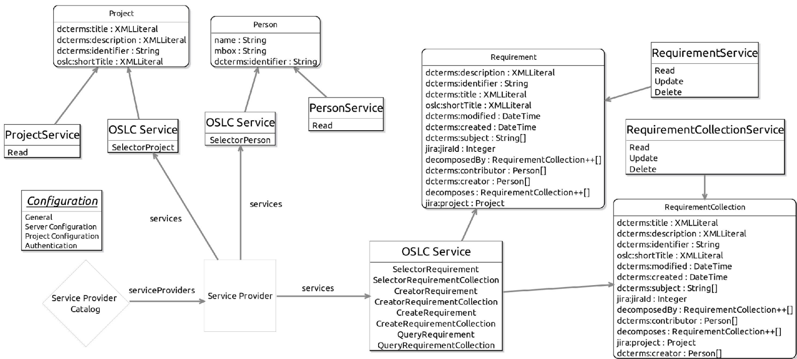
Figure 5.5: Jira Adaptor Functionality Diagram (Exported from Iryo modeling tool)
