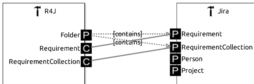
Figure 5.4: Adaptor Interfaces Diagram (P – produces, C – consumes)
