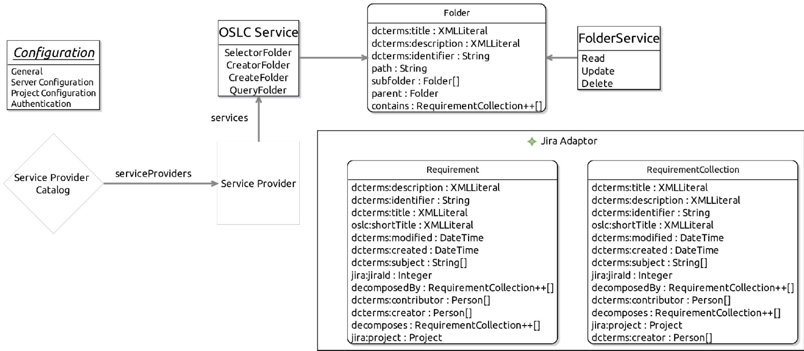
Figure 5.6: R4J Adaptor Functionality Diagram (Exported from Igo modeling tool)
