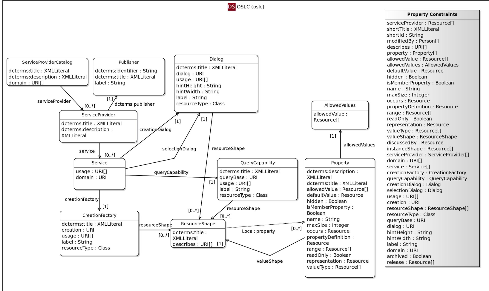
Figure 5.1: OSLC Core Domain Model Diagram (Exported from Igo modeling tool)
