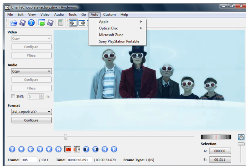
Obr. 3.2: Program Avidemux
