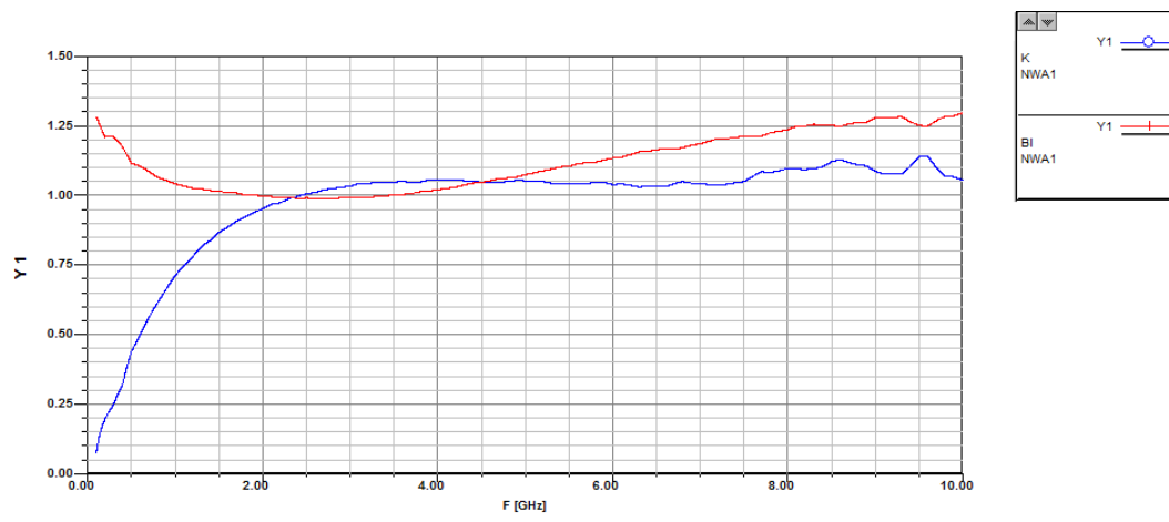
Obr. A.1: Stabilita ATF 54143
