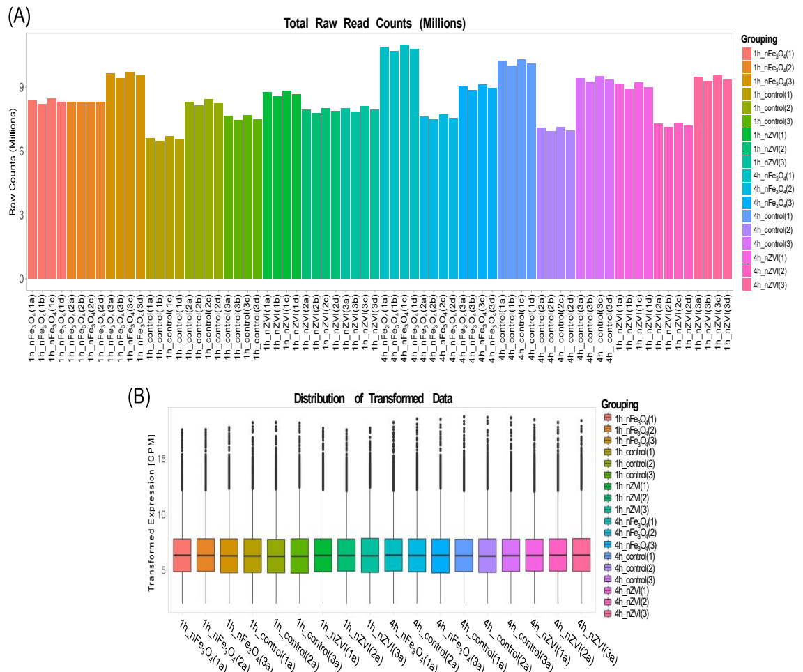
Figure 33. The transcript abundance in Raphidocelis subcapitata ATCC 22662 after the exposure of nFe 3 O 4 and nZVI. (A) Total raw read counts (millions) from all samples. (B) Transcript abundances from all time points expressed in CPM values. The black horizontal line in the box-whisker plot represents median value, the black horizontal line separating the upper and lower box represent the interval between first and third quartiles, the two whiskers indicate 1.5× interquartile range respectively and the black dots are the outliers. NOTE: Idep makes a filtering before it starts further calculations, that represents the converted count data. CPM (Counts Per Million) are obtained by dividing counts by the library count sum and multiplying and the results by a million. Control = R. subcapitata without NPs exposure.
