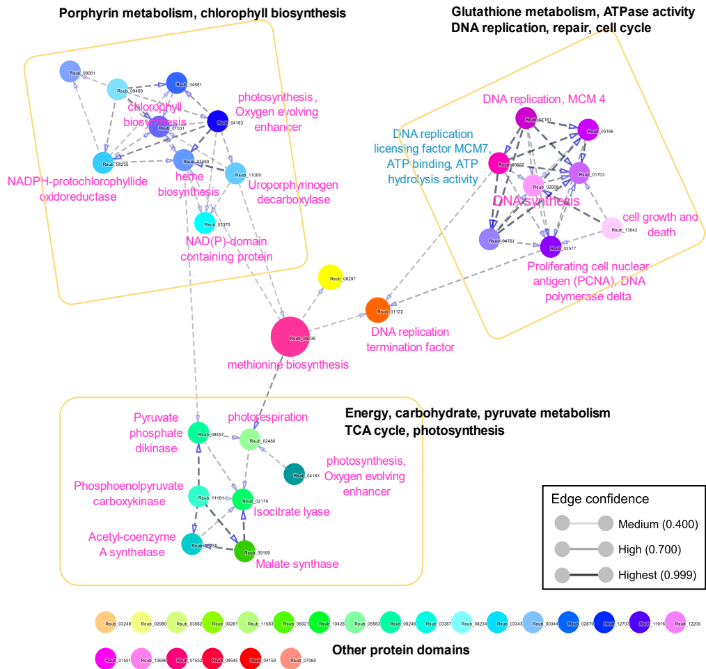
Figure 41. Co-expression analysis of top 50 DEGs for protein-protein interaction networks in R. subcapitata which responded to the treatment of nFe 3 O 4 and nZVI. Colors of the nodes represent a specific metabolic pathway or single protein domain: (i) blue nodes- Porphyrin metabolism, chlorophyll biosynthesis; (ii) purple nodes- glutathione metabolism, ATPase activity, DNA replication, repair and cell cycle; (iii) green nodes- energy, carbohydrate, pyruvate metabolism, TCA cycle, photosynthesis; (iv) multiple colors/nodes in a line- a group of protein domains whose function is unrelated to any of the metabolic pathways in this network. The thickness of the edges/lines connecting nodes indicate the strength of the data support as shown in the legend above. Each node represents a protein produced by a single gene locus. TCA cycle- tricarboxylic acid cycle
