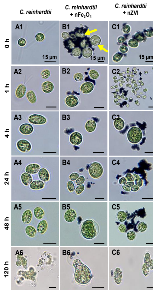
Figure 42. Microscopic image of C. reinhardtii exposed to nFe 3 O 4 and nZVI up to 120 h. (A) Untreated C. reinhardtii ; (B) C. reinhardtii exposed to 100 mg/L nFe 3 O 4 (C) C. reinhardtii exposed to 100 mg/L nZVI. Scale bar = as indicated in the pictures (15 μm).
