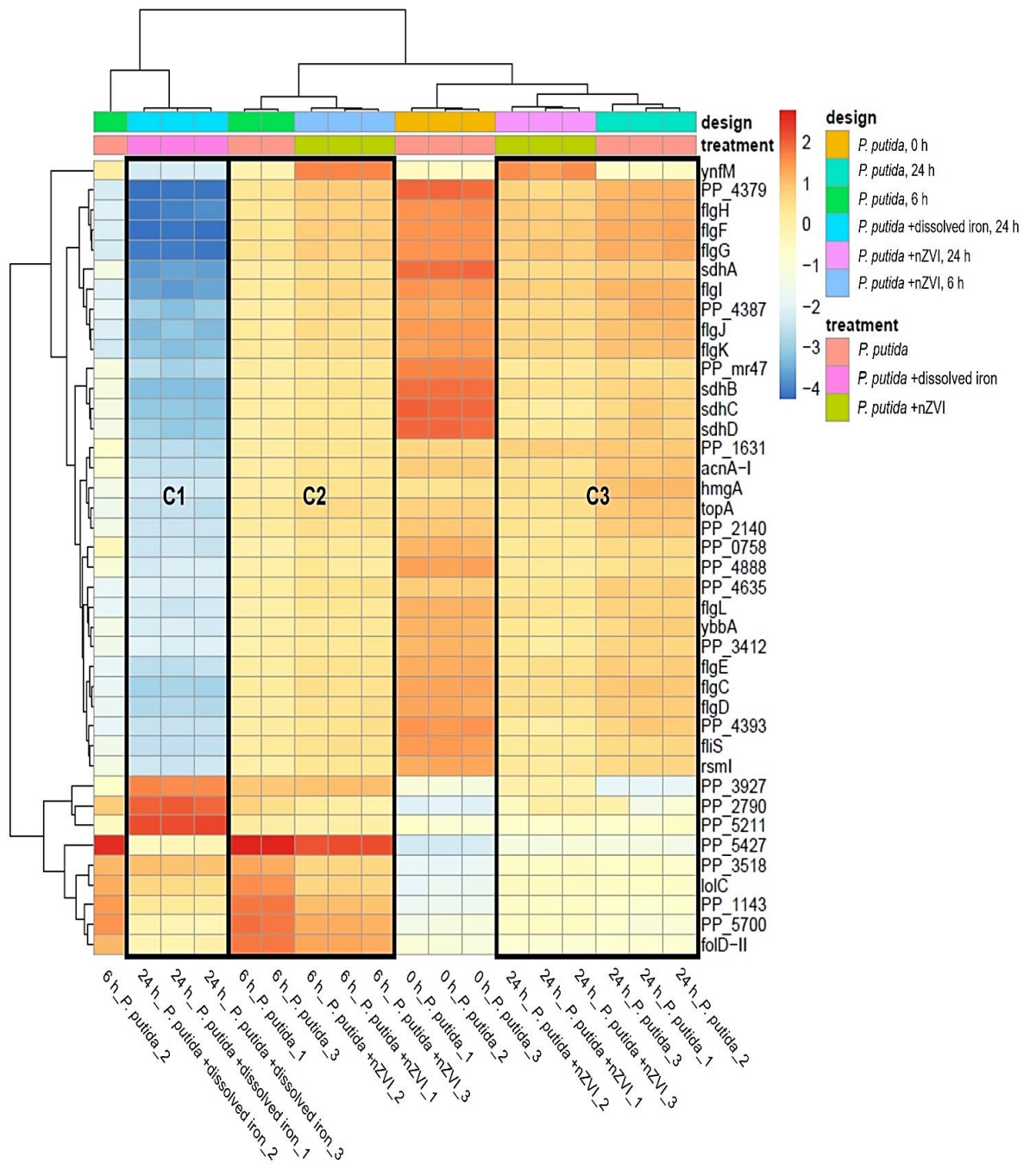
Figure 14. Heatmap of the top 30 DEGs in different exposure conditions. Hierarchical clustering of genes was based on the \log_2 -fold change, and the adjusted P-value was based on the 95% confidence interval. Cluster C1 contained the samples exclusively from P. putida in dissolved iron treatment at 24 h; cluster C2 represented the P. putida in nZVI treatment at 6 h, whereas cluster C3 consisted of the samples of P. putida in nZVI at 24 h. Relative gene expression is indicated by the color scales: elevated gene expression higher than zero indicates upregulation in control (red), reduced gene expression, shown in blue, less than
