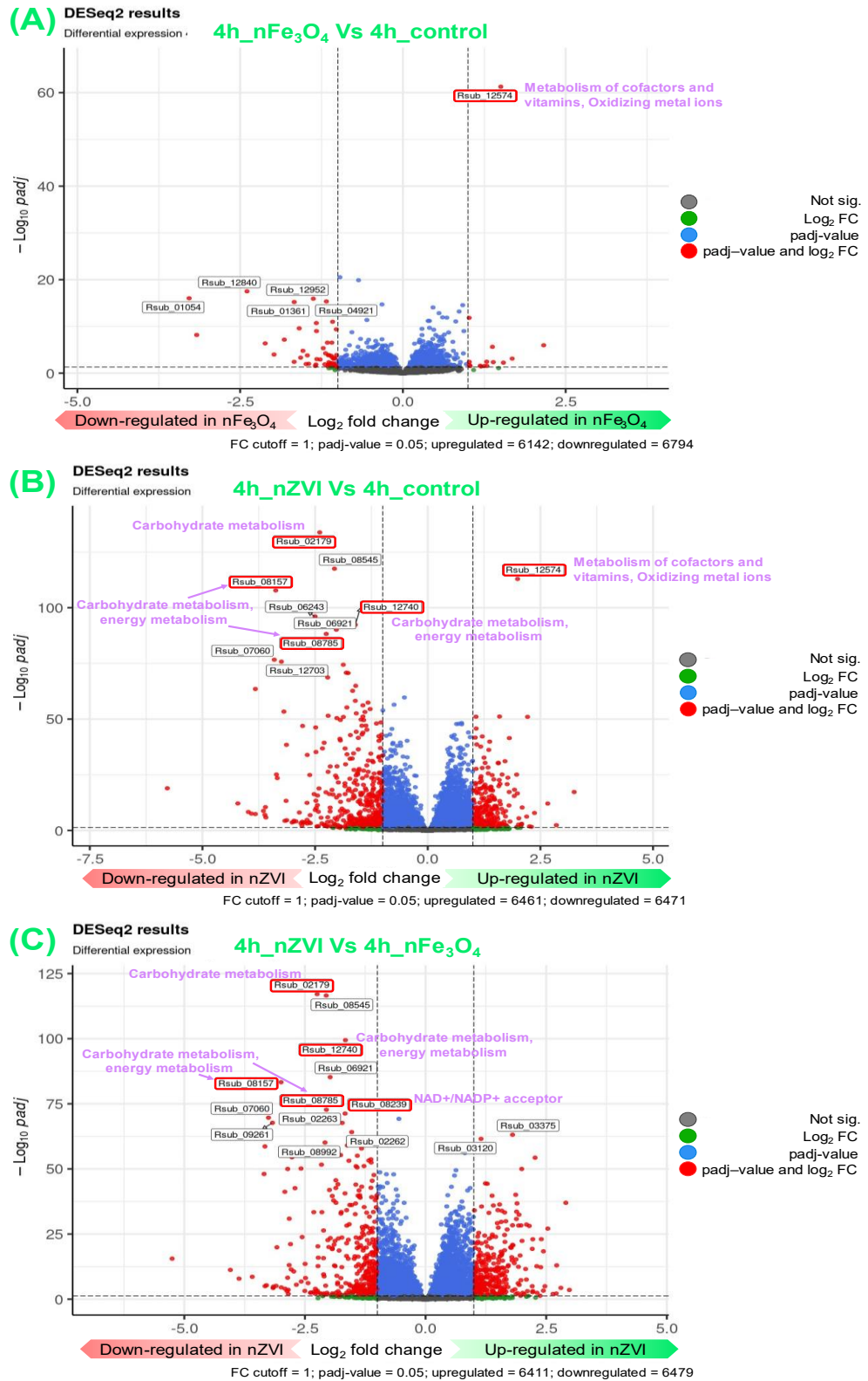
Figure 36. Volcano plots of all the expressed genes in three treatment groups after 4 h exposure. (A) nFe 3 O 4 vs control (B) nZVI vs control (C) nZVI vs nFe 3 O 4 . X-axis represents the log 2 (FC)
