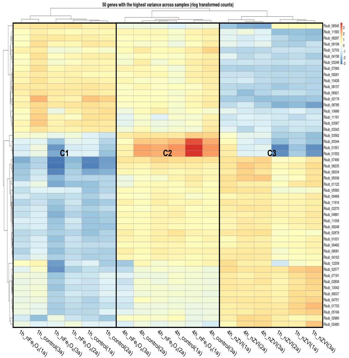
Figure 38. Heatmap of the top 50 DEGs in different exposure conditions. Hierarchical clustering of genes was based on the log 2 -fold change, and the adjusted P-value was based on the 95% confidence interval. Cluster C1 contained the samples from R. subcapitata in nFe 3 O 4 treatment and control condition at 1 h; cluster C2 represented the R. subcapitata in nFe 3 O 4 treatment and control condition at 4 h, whereas cluster C3 consisted of the samples of R. subcapitata in nZVI at 1 and 4 h. Relative gene expression is indicated by the color scales: elevated gene expression > 0 indicates upregulation in treatment conditions ( R. subcapitata in nZVI or nFe 3 O 4 ) (red), reduced gene expression, shown in blue, < 0 indicates upregulation in control. Control was R. subcapitata only. See Table 9 for details.
