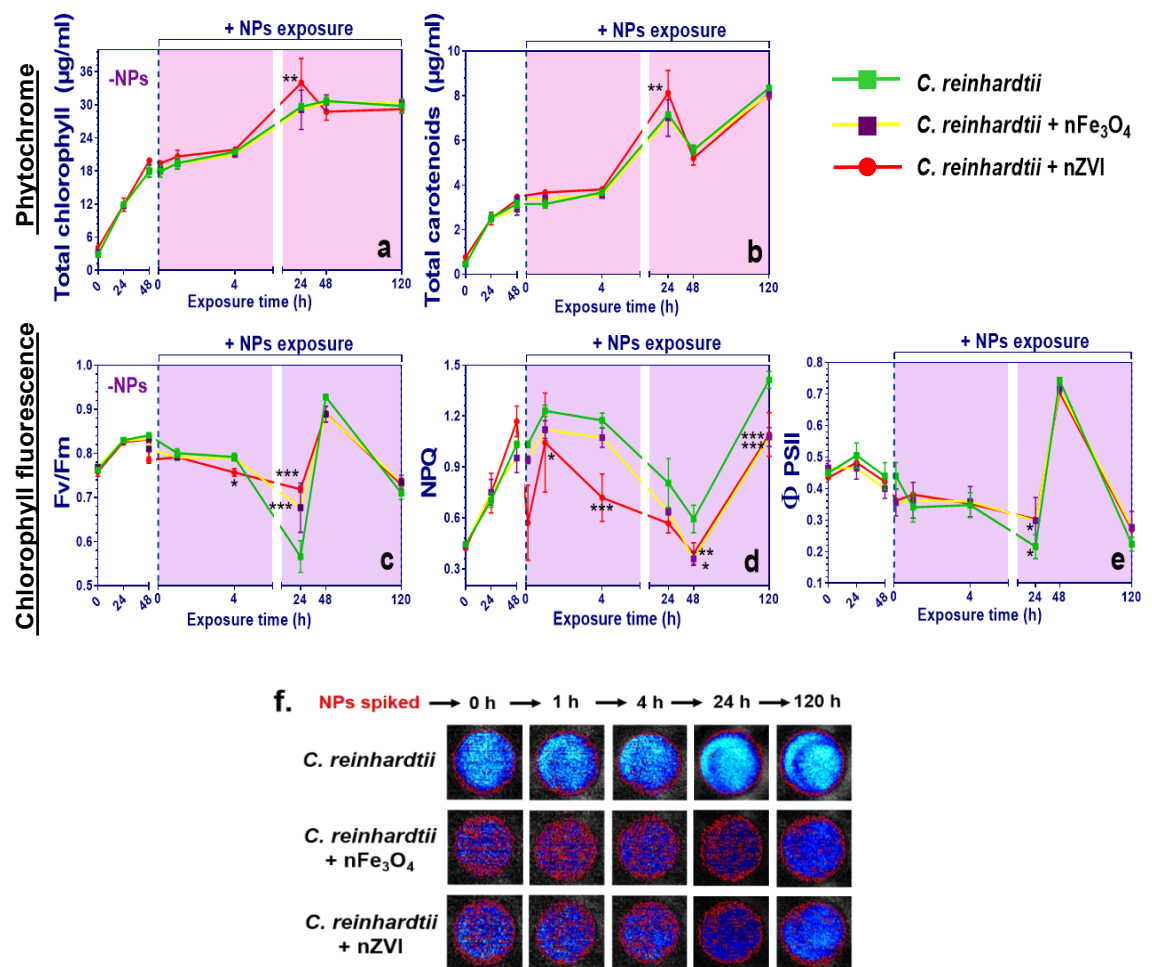
Figure 43. Phenotypic responses of C. reinhardtii exposed with nZVI and nFe 3 O 4 in HSM. (A, B) Phytochrome content (Total chlorophyll and carotenoid); (C, D, E) Chlorophyll fluorescence [Maximum PSII yield (F v /F m ), non-photochemical quenching (NPQ), effective PSII yield (Φ PSII)] (mean ± SD; n = 3); (F) Light intensity of chlorophyll fluorescence imaged under FluorCam FC 800-C Video Imager. *= level of significance changes were compared to untreated
