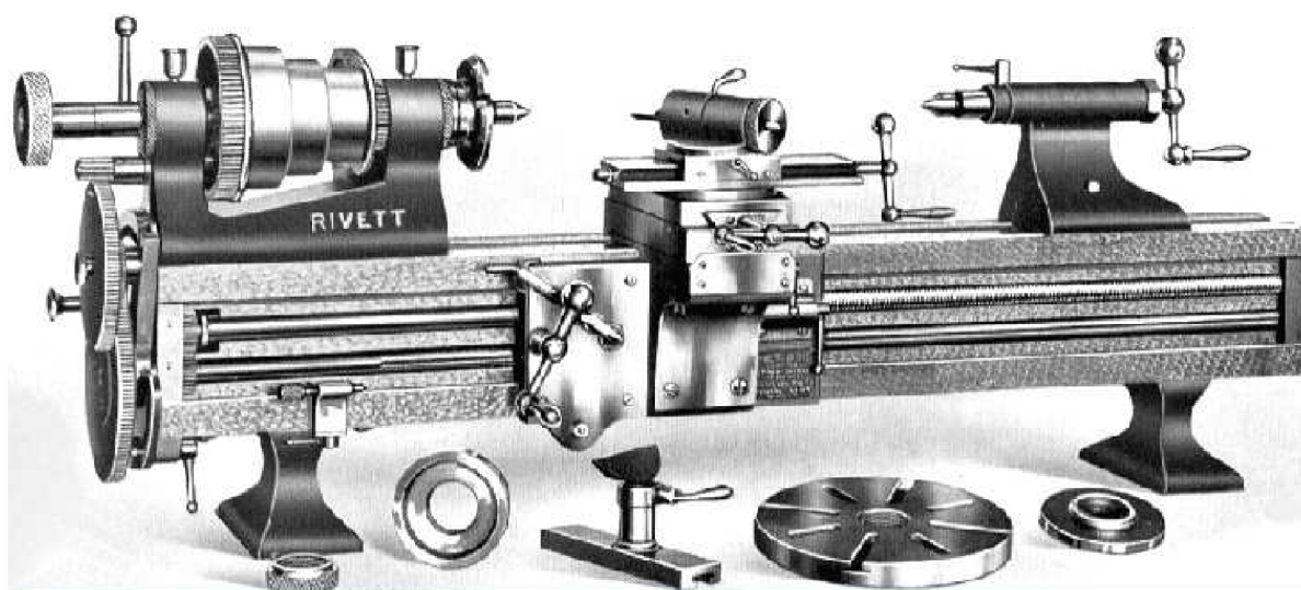
Obr. 5: Rivett 8" Precision (1908) [9]
