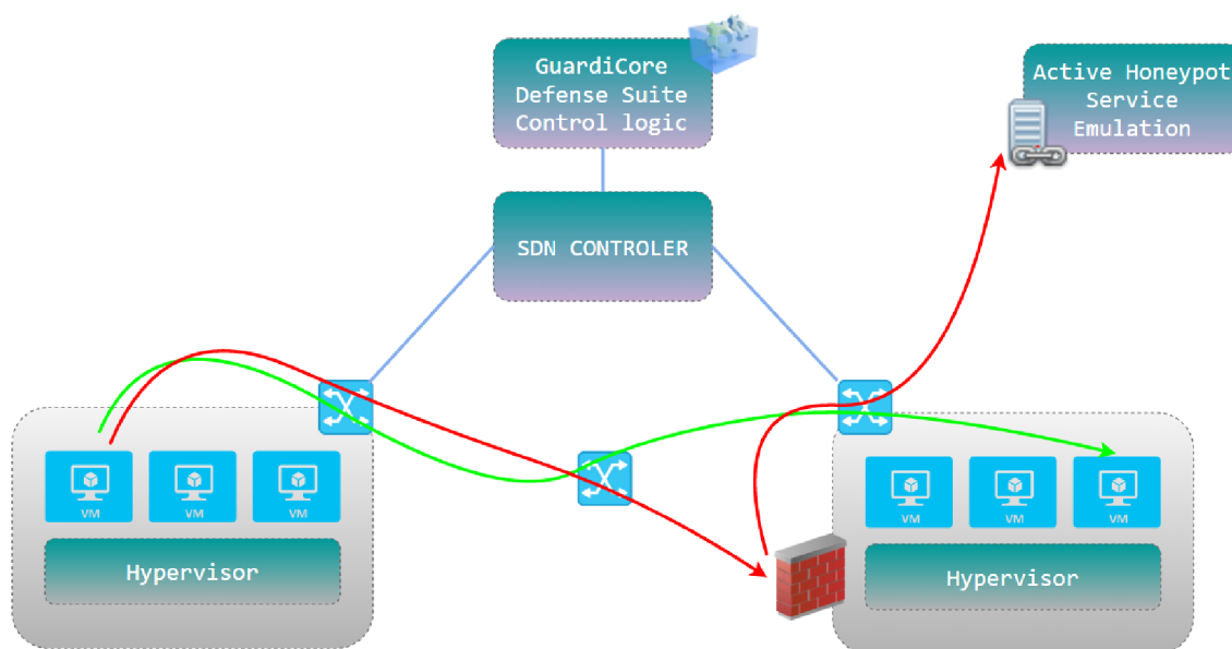
Obr. 2.14: Honeypot [9]
