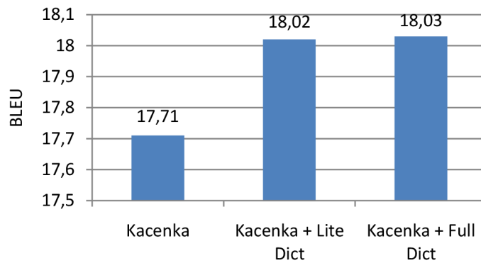
Figure 3.3 Adding a dictionary into the training data of the Kacenska corpus 54
