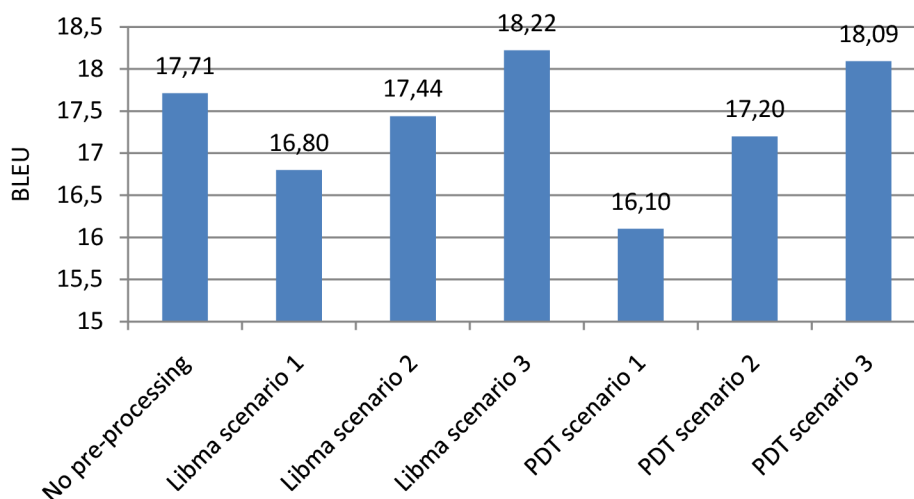
Figure 3.6 Morphological pre-processing of the Kacenska corpus 63
