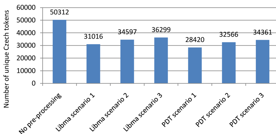
Figure 3.9 Number of unique Czech tokens in the training set of Acquis after morphological pre-processing
