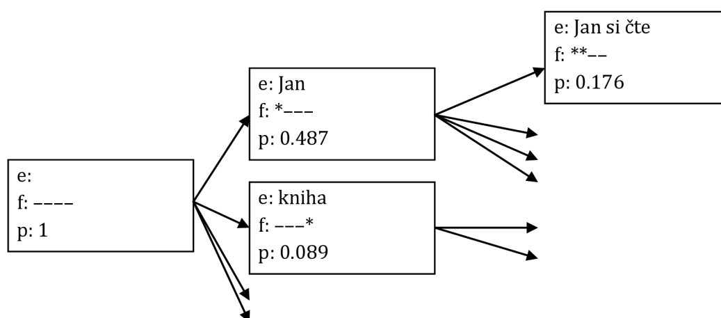
Figure 1.4 Generation of hypotheses
