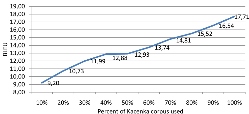
Figure 3.1 Relation between the size of the Kacenska corpus and the resulting BLEU 51
